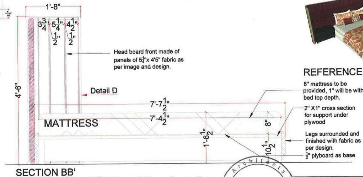
BED - PLAN
