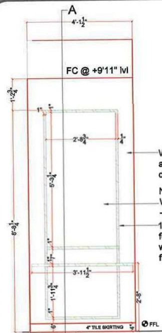
TEMPLE WALL ELEVATION
