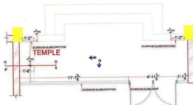
PLAN FOR ENTRY
