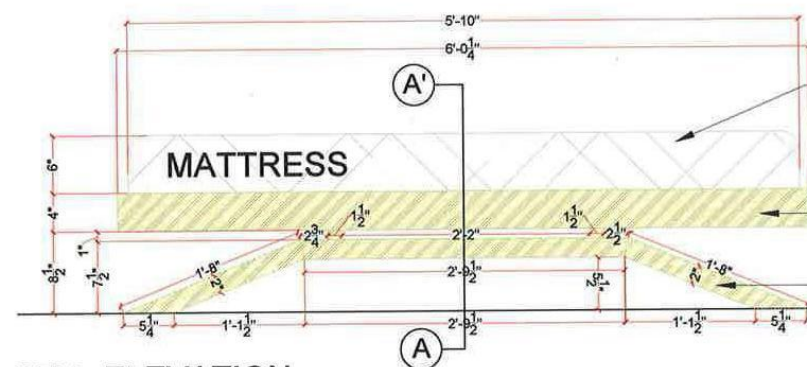
BED- ELEVATION
