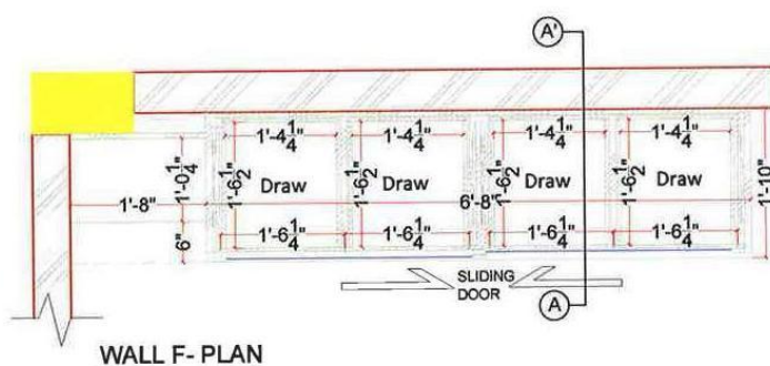
WALL F- PLAN
