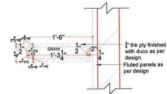
SECTION CC'
