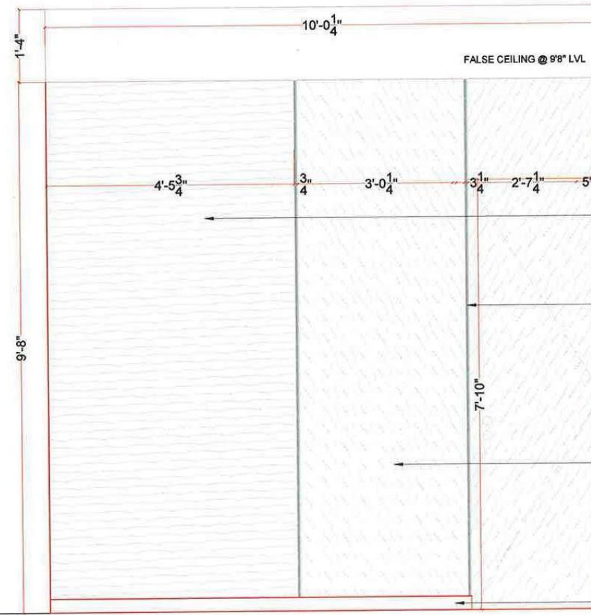
WALL D- ELEVATION
