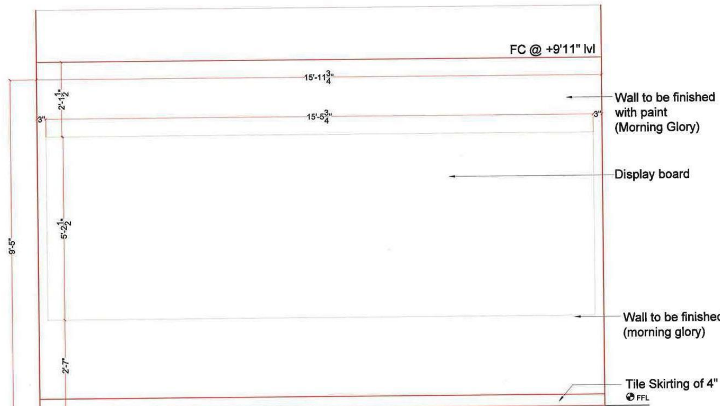
WALL K - ELEVATION
