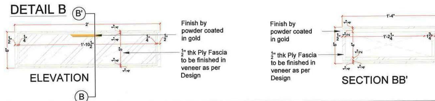
DETAIL B - REFERENCE
