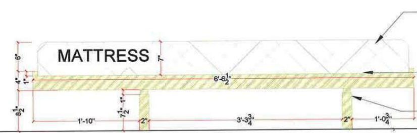
SECTIONAL AA'
