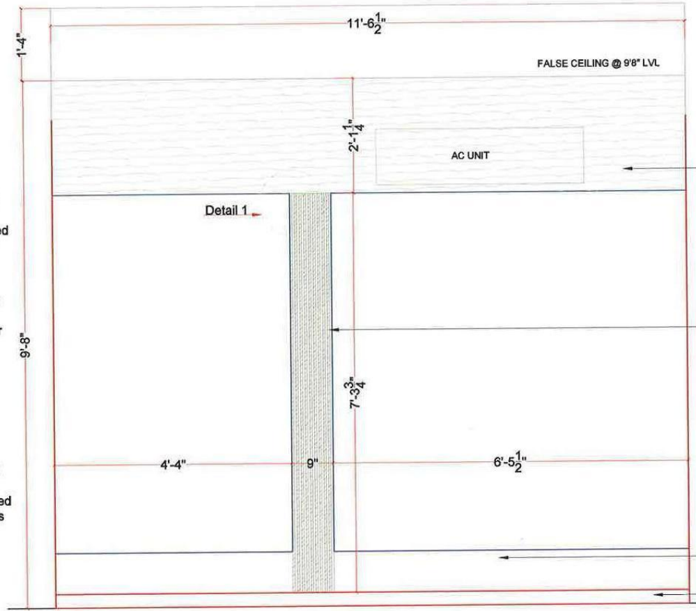
WALL E- ELEVATION
