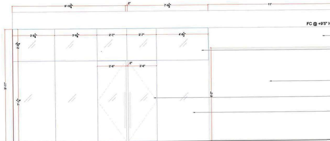
WALL D - ELEVATION
