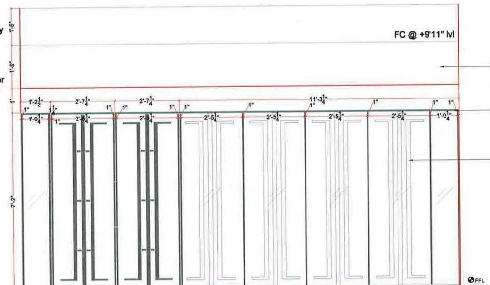
WALL N - ELEVATION
