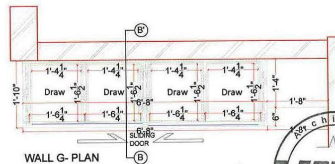
WALL G- PLAN
