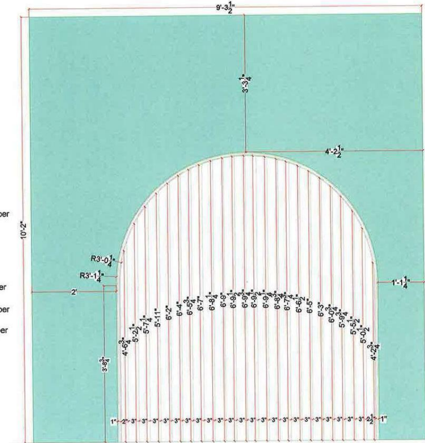
DETAIL C
