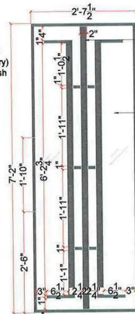
DETAIL E - MAIN DOOR
