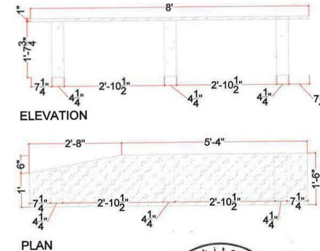
DETAIL B
