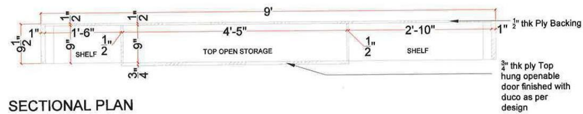
DETAIL F
