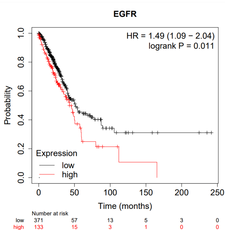
Fig 3 : Survival Plot
