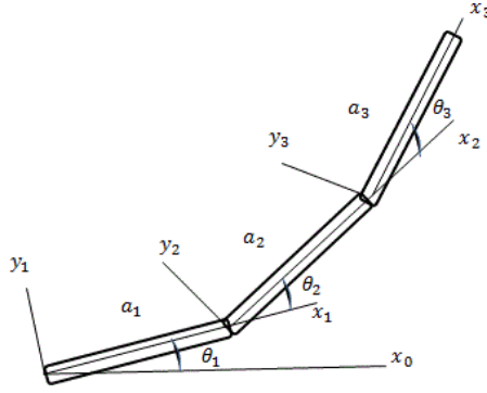
Fig. 2 Coordinate frames of different links
