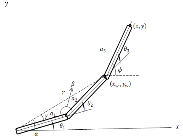
Fig. 3 Planar Robotic Arm
