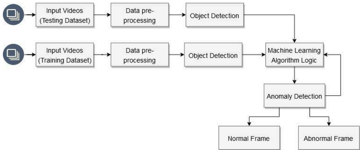
Fig.4.1: Algorithmic Flowchart of Program
