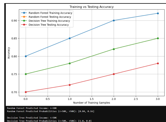
Fig - Model Accuracy (Train vs Test)
