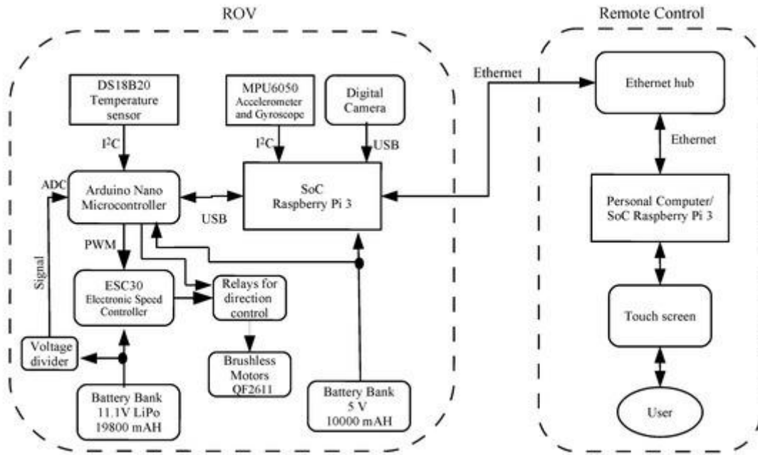
(4.1.3)SENSORS FLOWCHART
