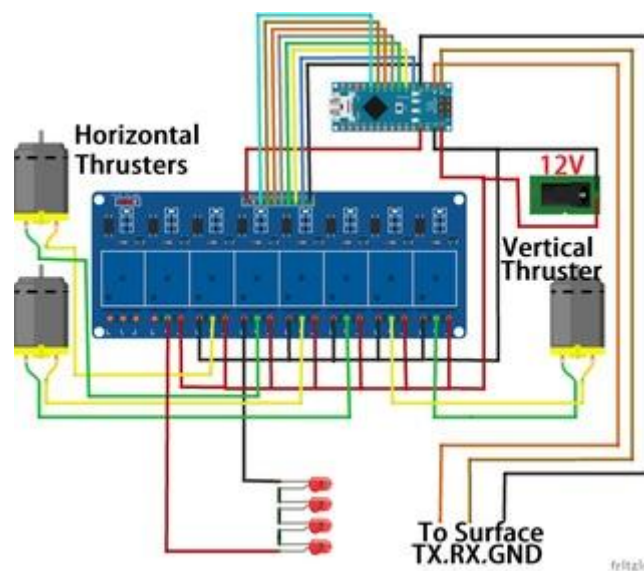
(4.1.3)CIRCUIT CONNECTION OF THRUSTERS
