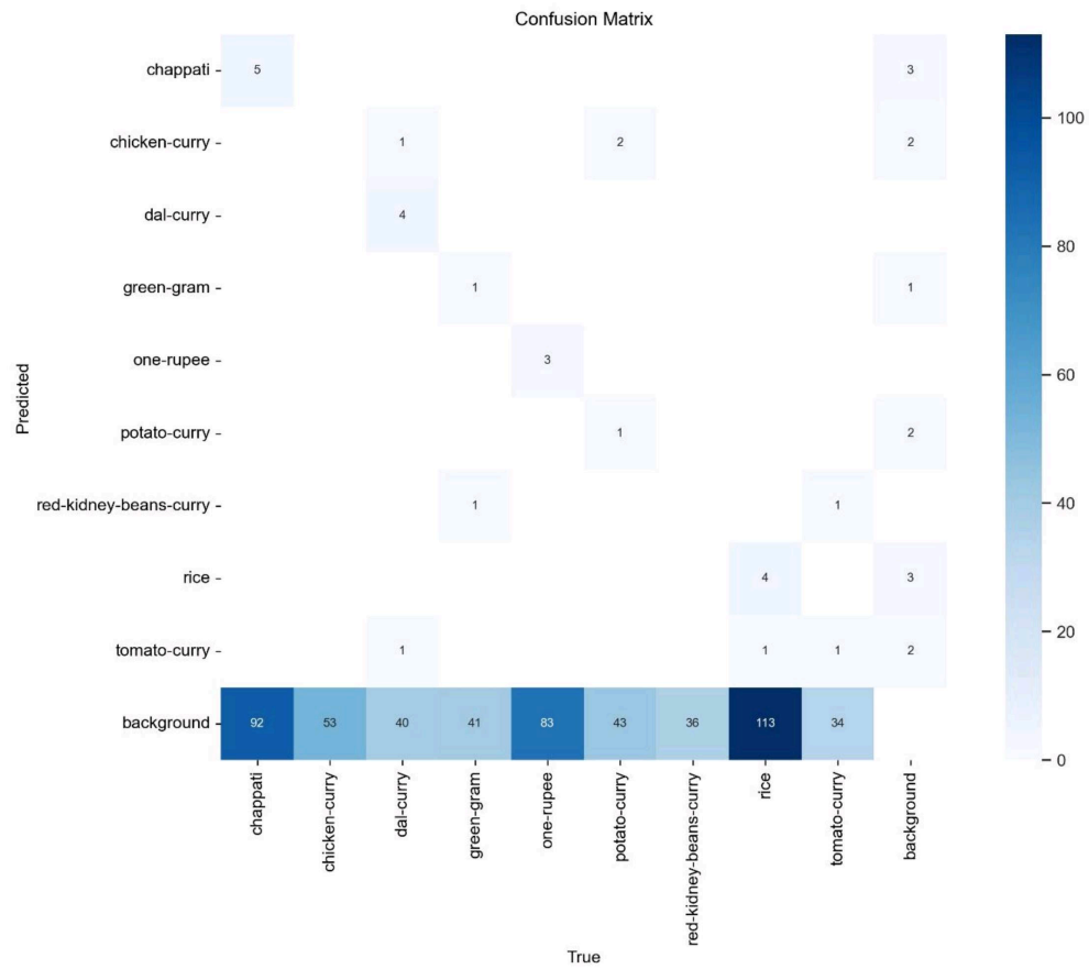
4.9 Confusion Matrix
