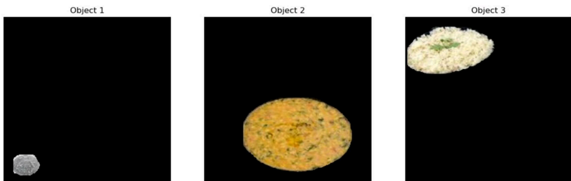
4.6 Food segmentation
