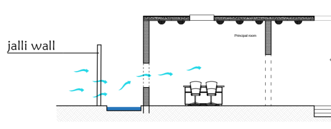
Fig 5.7: Passive down draft evaporative cooling
