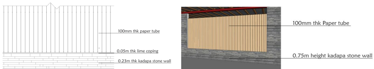
Fig 5.10(a),(b): Construction of wall system
