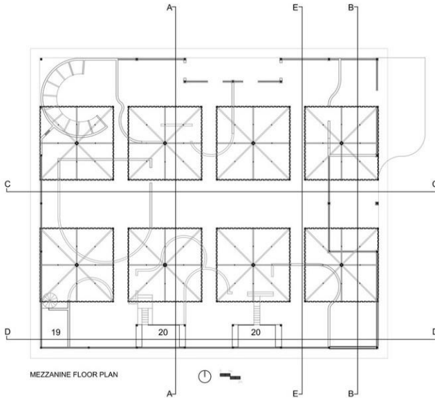
Fig 2.2: Structural pain of atelier school
