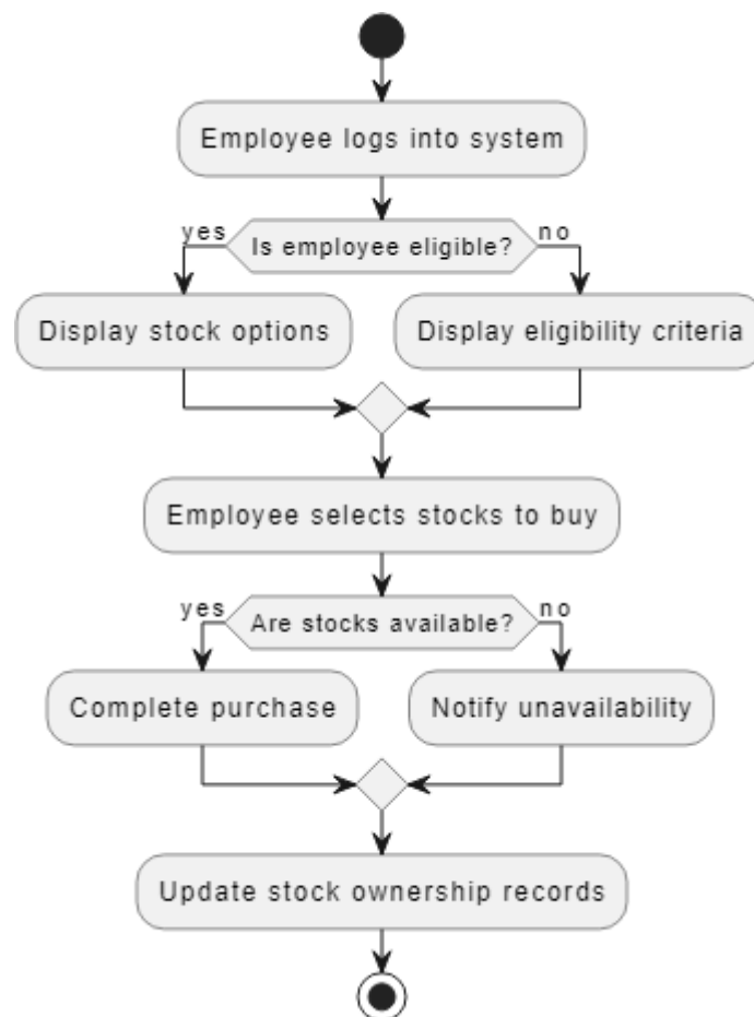
Fig 3.4 Activity Diagram
