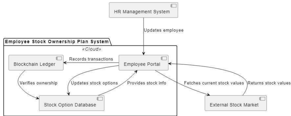
Fig 3.2 Context Diagram
