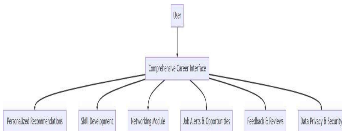
Fig 4.2: System Architecture
