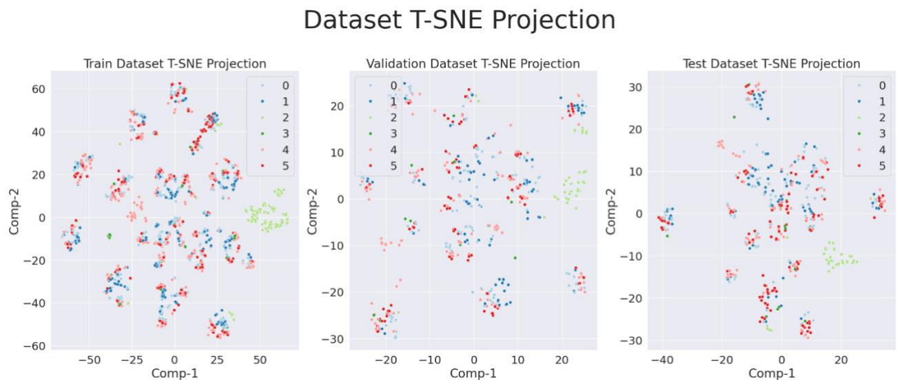
Fig 16 - Dataset T-SNE Projection(T-distributed Stochastic Neighbour Embedding)
