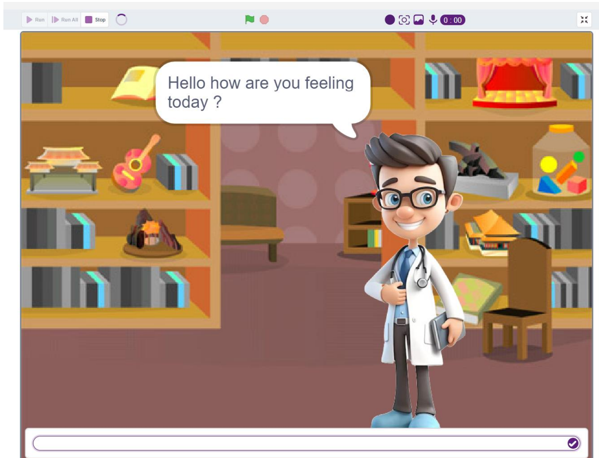
Figure 4.7 - Chatbot
