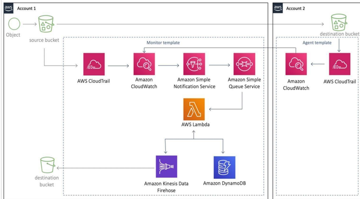
Fig 4.1.1 ideation map
