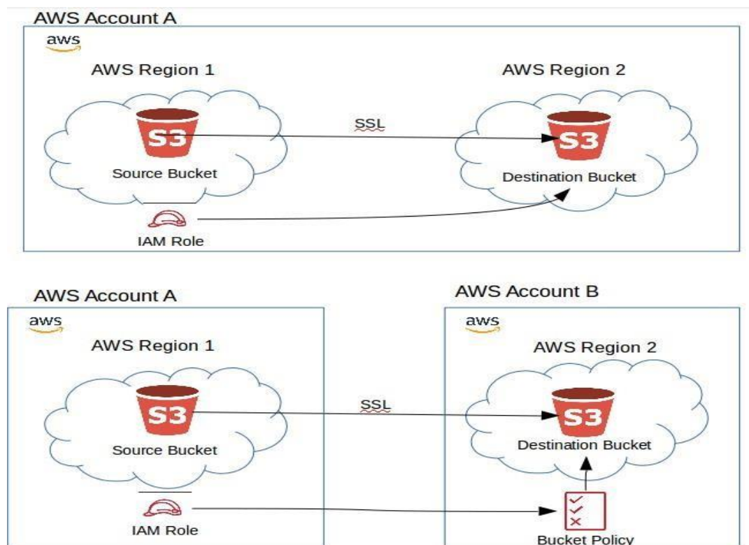
Fig 3.1.2 software requirement
