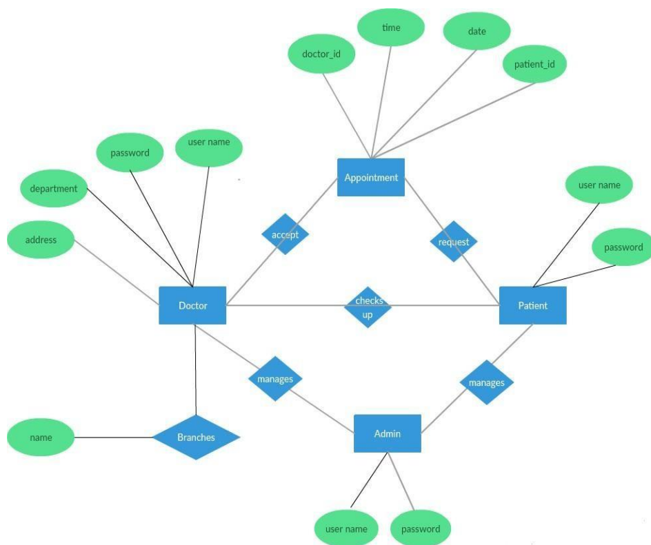
Figure 4.3:ER Diagram
