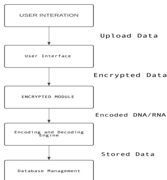
Fig 4.1: Architecture of Geneprotect process
