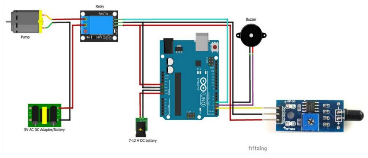
Fig:2.1: Proposed System Architecture
