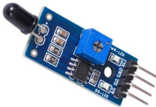
Fig:2.3: Flame Sensor Module
