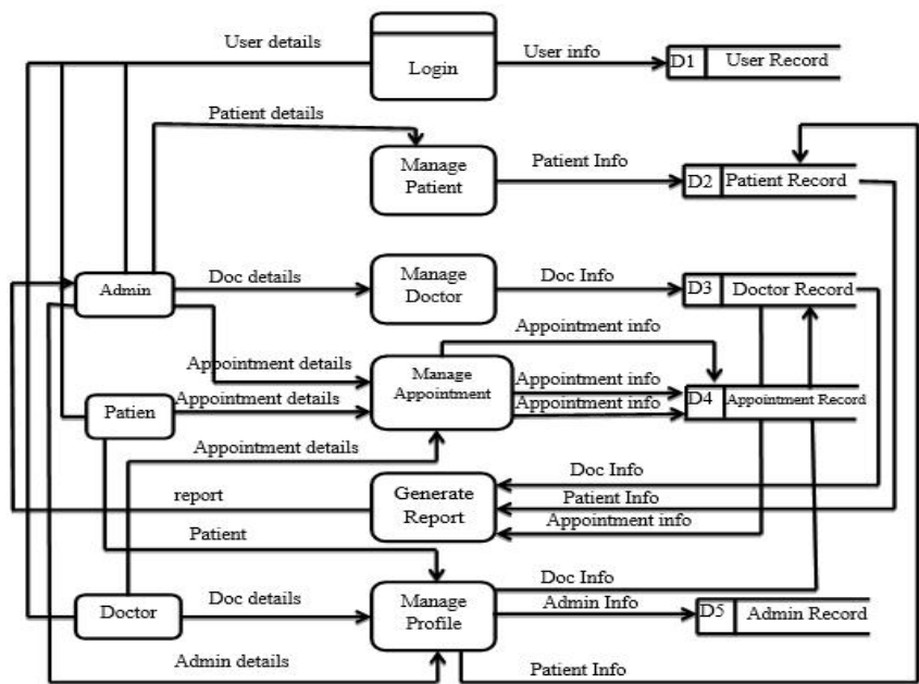
Fig2.1 Architecture Diagram
