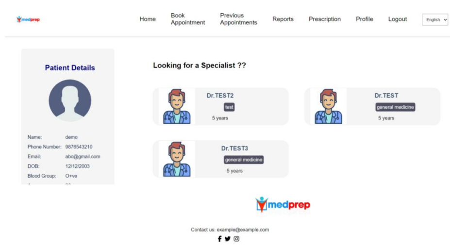
Fig2.3 User Dashboard
