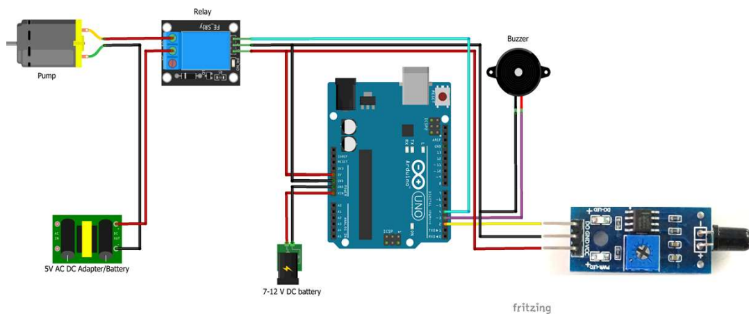
Fig:2.1: Proposed System Architecture
