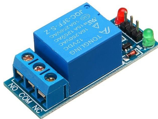
Fig 2.5 Relay Module
