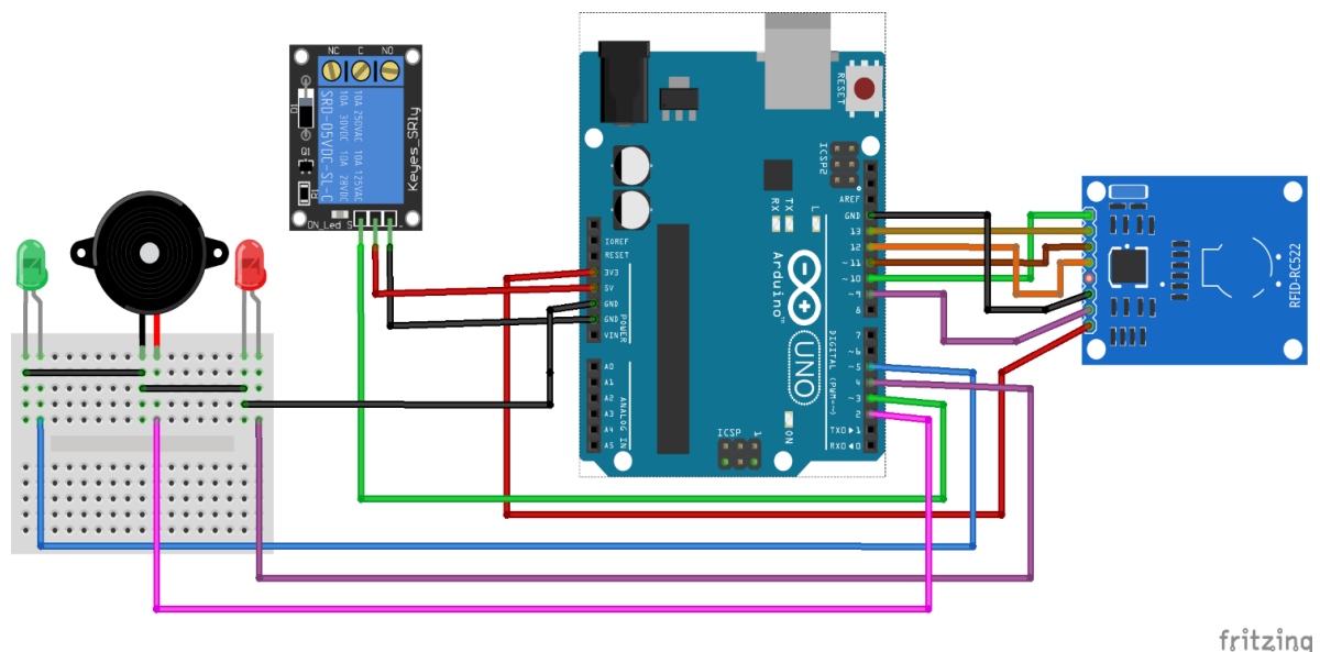
Fig 2.1 Architecture Diagram of smart door lock
