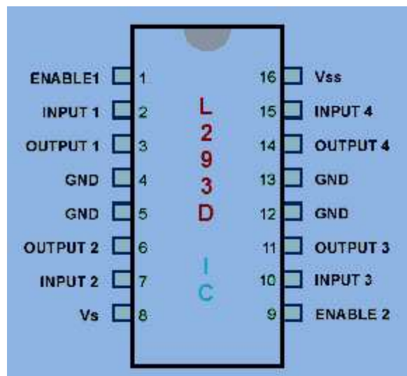
Fig 4.9 L293D IC Pin Configuration
