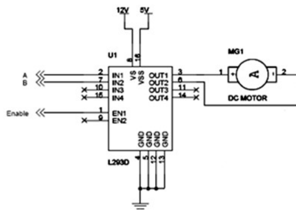
Fig:4.12 Dc Motor Interfaced With L293D Microcontroller
