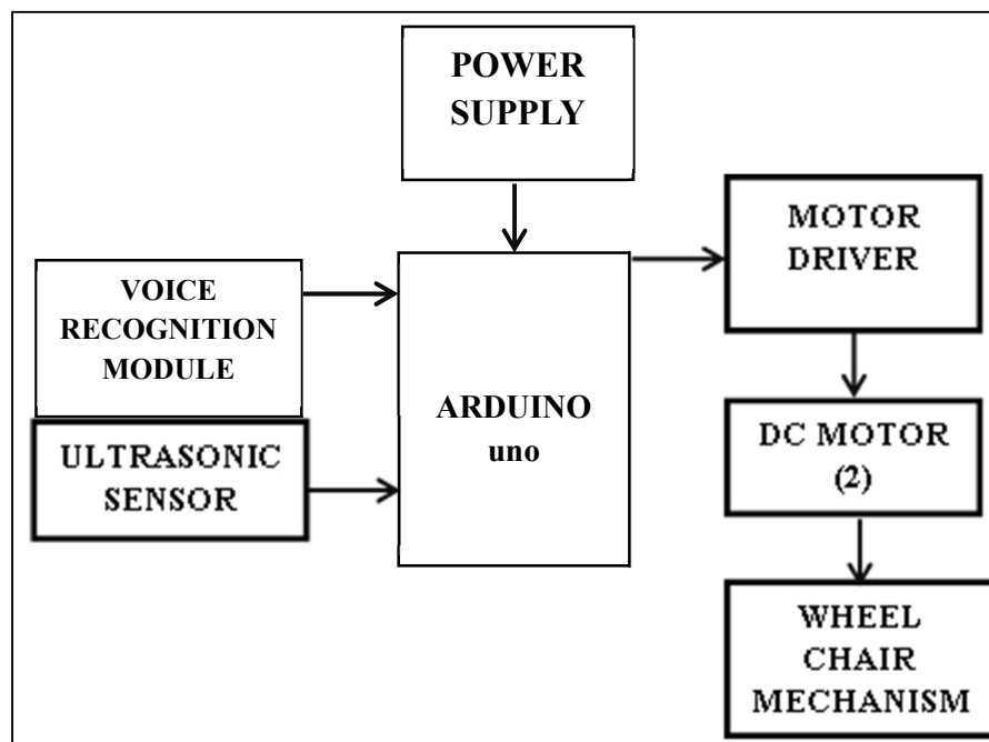
Fig:3.2 VOICE CONTROLLING WHEEL CHAIR
