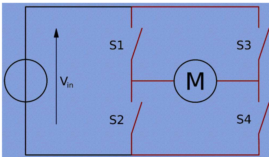
Fig 4.8 H-BRIDGE CIRCUIT
