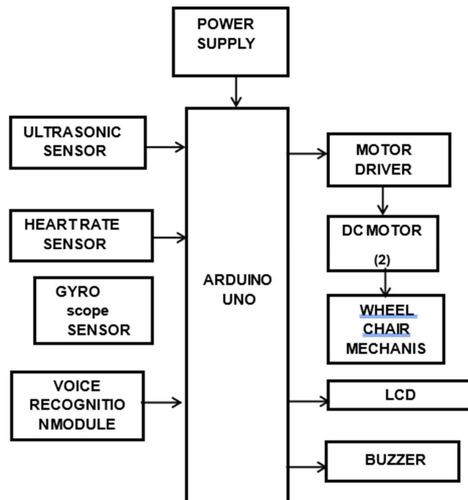
Fig:3.1 BLOCK DIAGRAM
