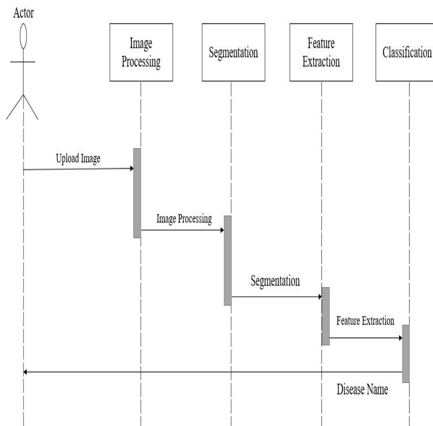
FIG 4.6.4 SEQUENCE DIAGRAM
