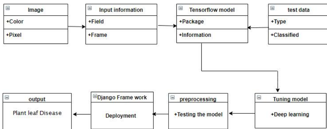
FIG 4.6.3 CLASS DIAGRAM
