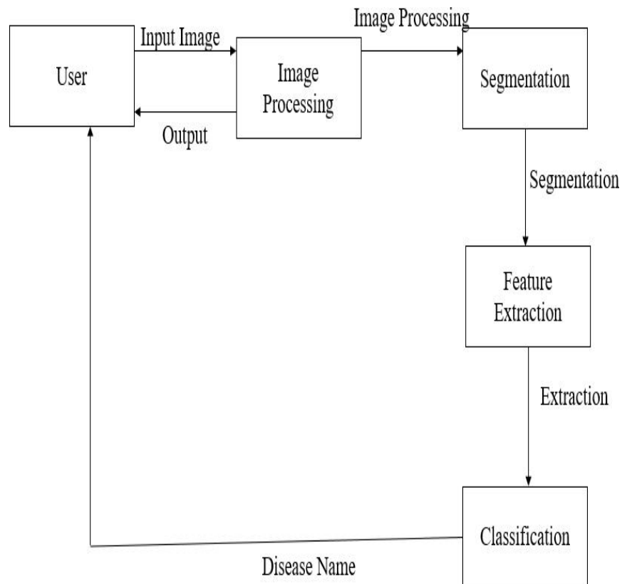
FIG 4.6.5 COLLABORATION DIAGRAM
