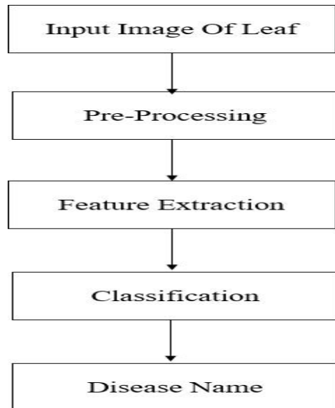
FIG 4.6.6 ACTIVITY DIAGRAM
