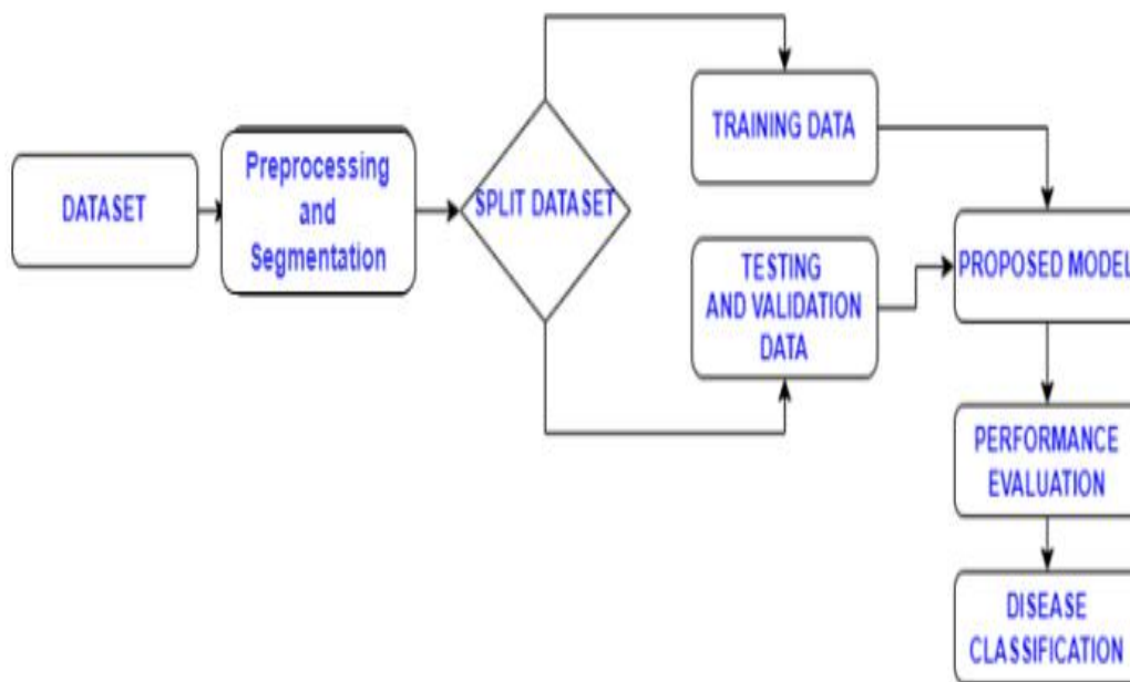
Fig 4.4.1: System Architecture
