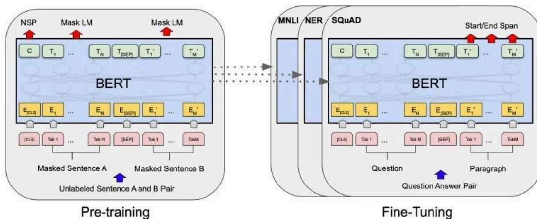
Fig No:2.2.1 Pre-training & Fine-Tuning for Bert model
