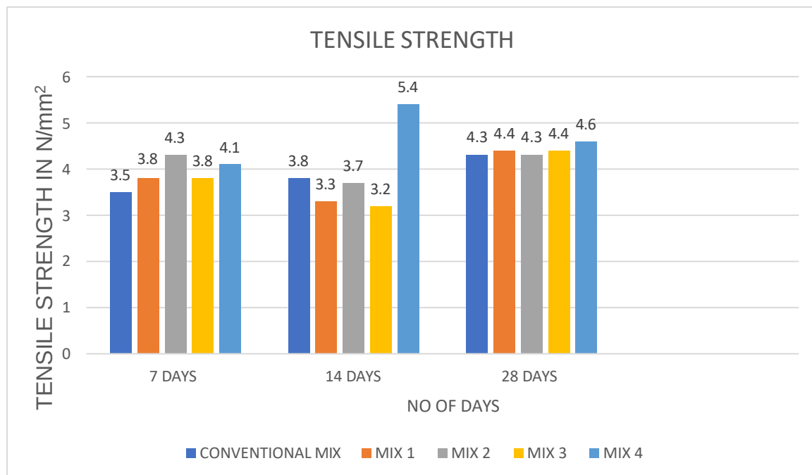
GRAPH 6.1.2: Tensile Strength Comparison Chart.
