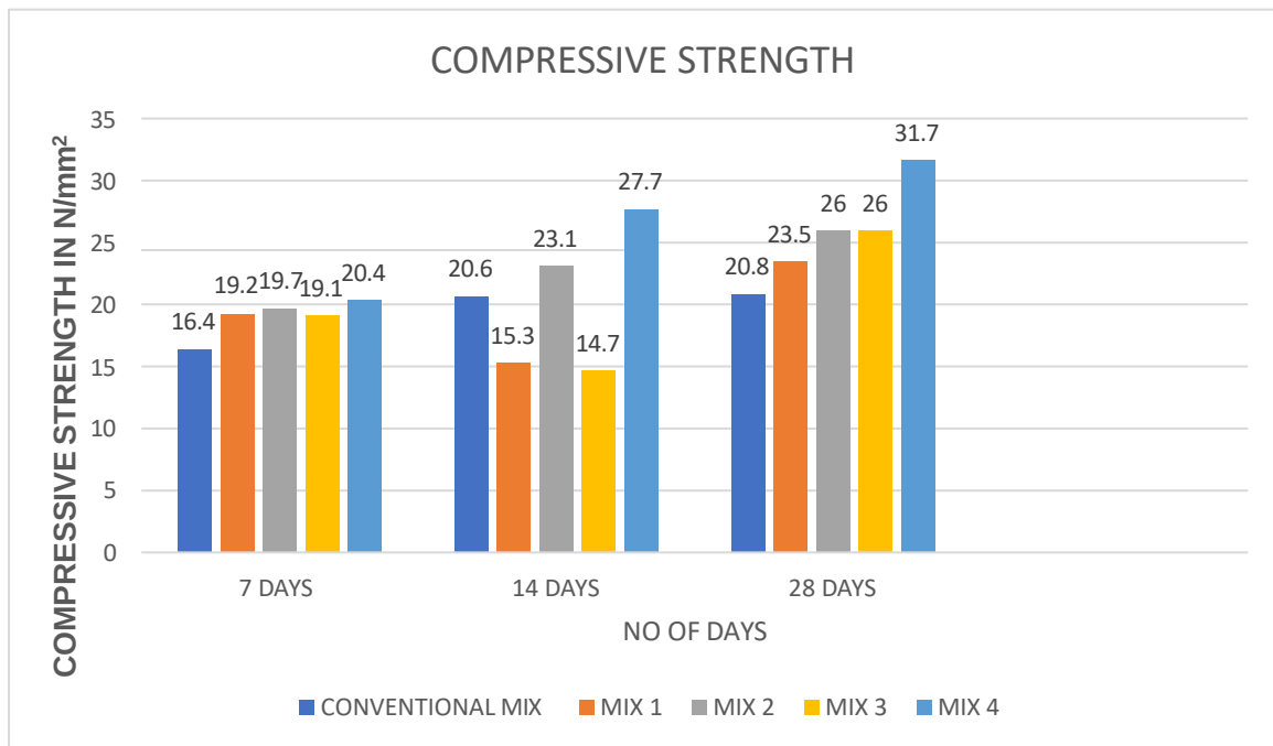
GRAPH 6.1.1: Compressive Strength Comparison Chart
