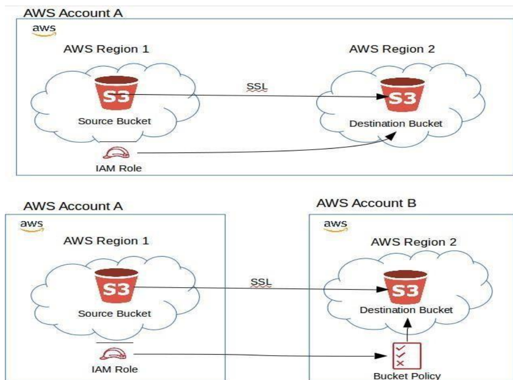
Fig 3.1.2 software requirement
