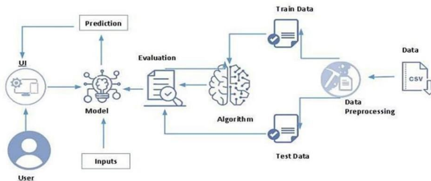
Fig 1.1.1 : Architecture Diagram
