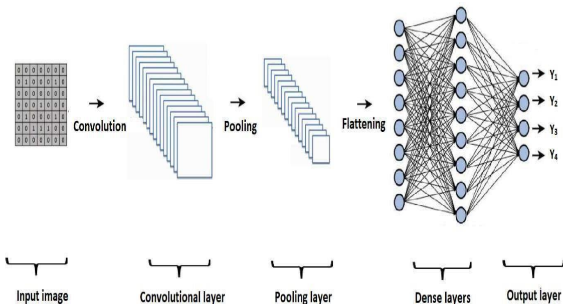
Fig 3.4.2 Representation of the architecture of a convolutional neural network
