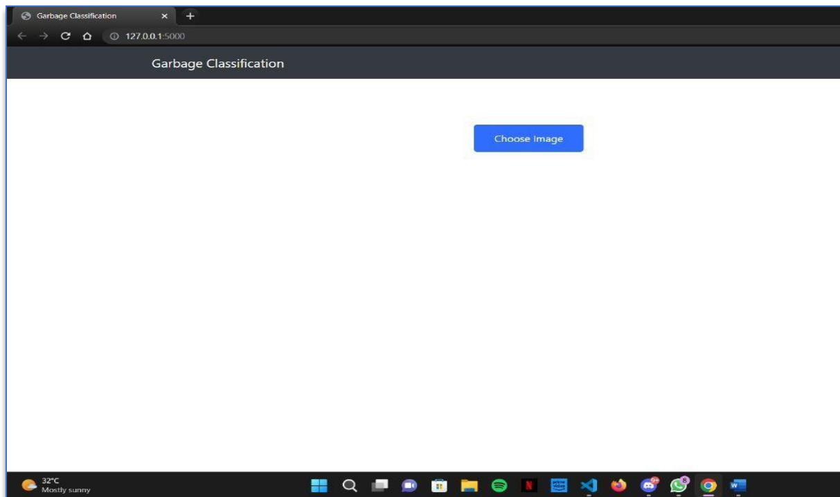
Fig 4.1 Home Page
