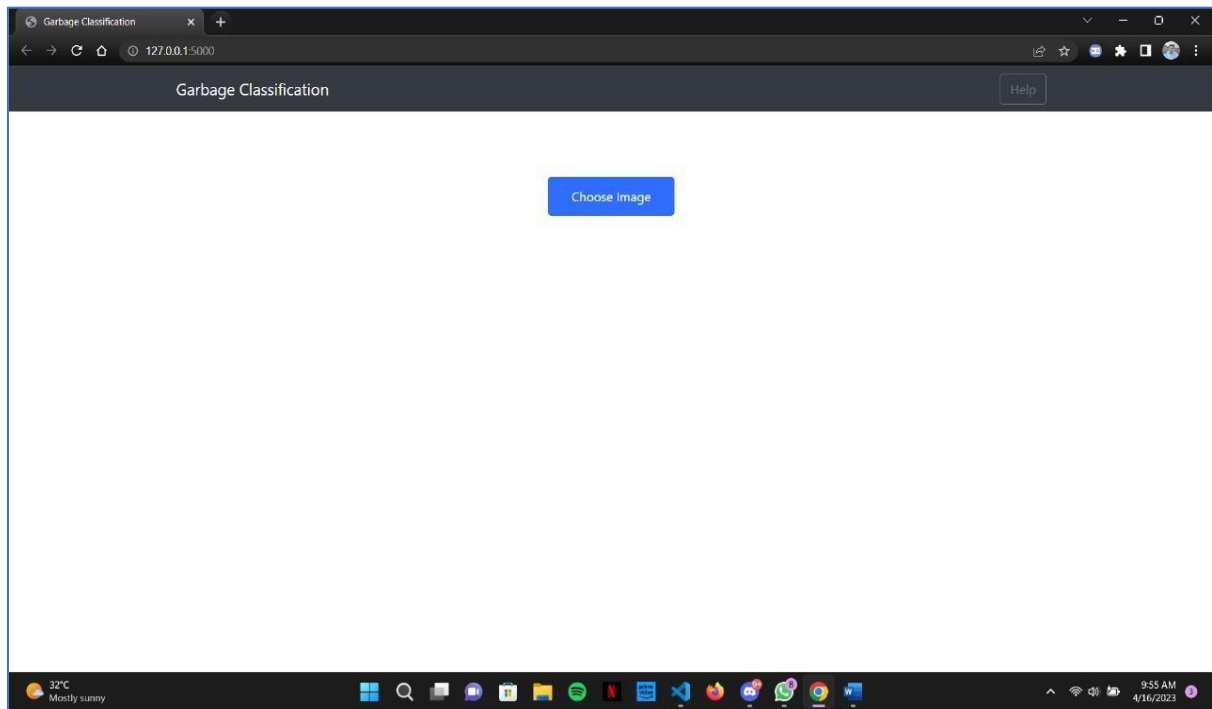
Fig 4.2 Choosing Image
