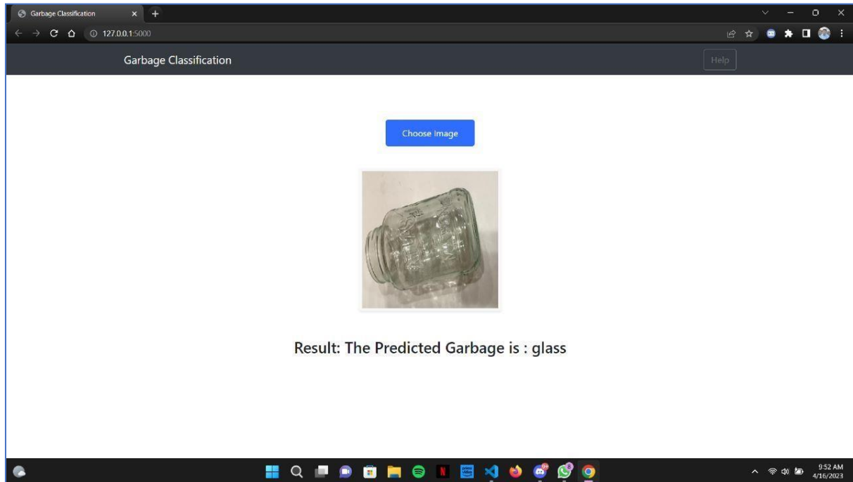
Fig 4.4 Predicted Output
