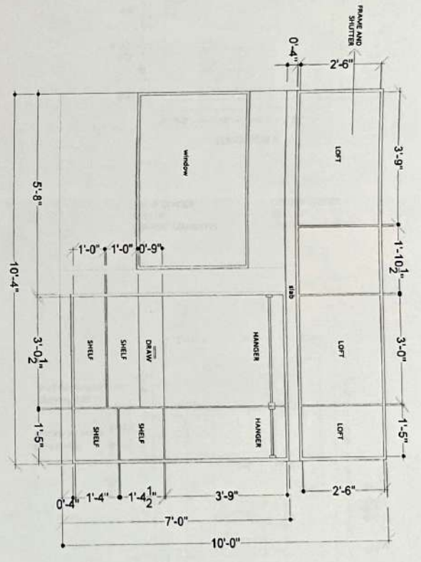
GUEST BEDROOM WARDROBE (INNER DETAIL)
