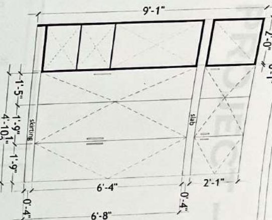
ELEVATION 2 (SHUTTER DETAIL)
