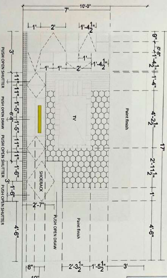
TV Unit Inner Detail
