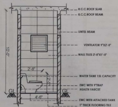
WALL DD' - SECTIONAL ELEVATION
