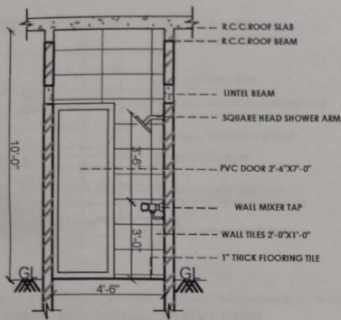
WALL BB' - SECTIONAL ELEVATION
