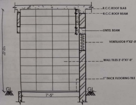
WALL AA' - SECTIONAL ELEVATION
