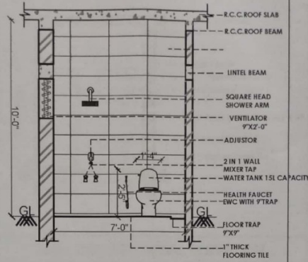
WALL CC' - SECTIONAL ELEVATION
