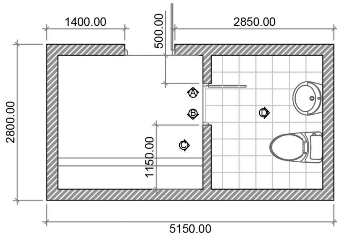
RESTROOM LAYOUT
