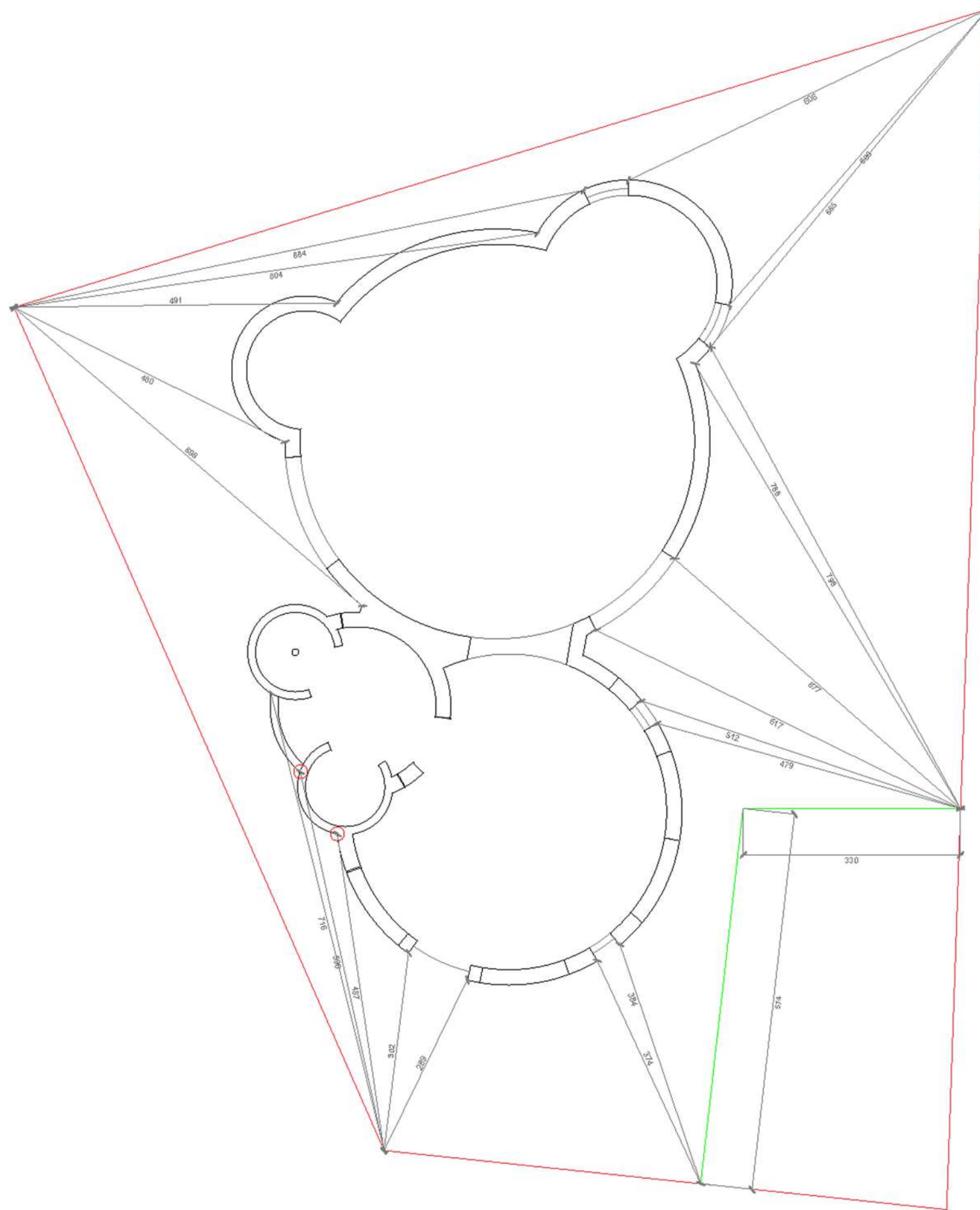
AS BUILT DIMENSION
