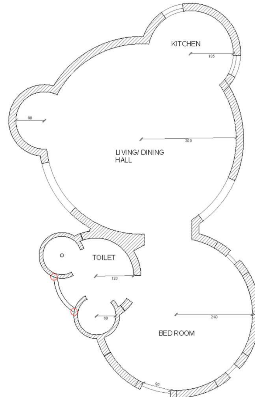
PLAN GROUND FLOOR
