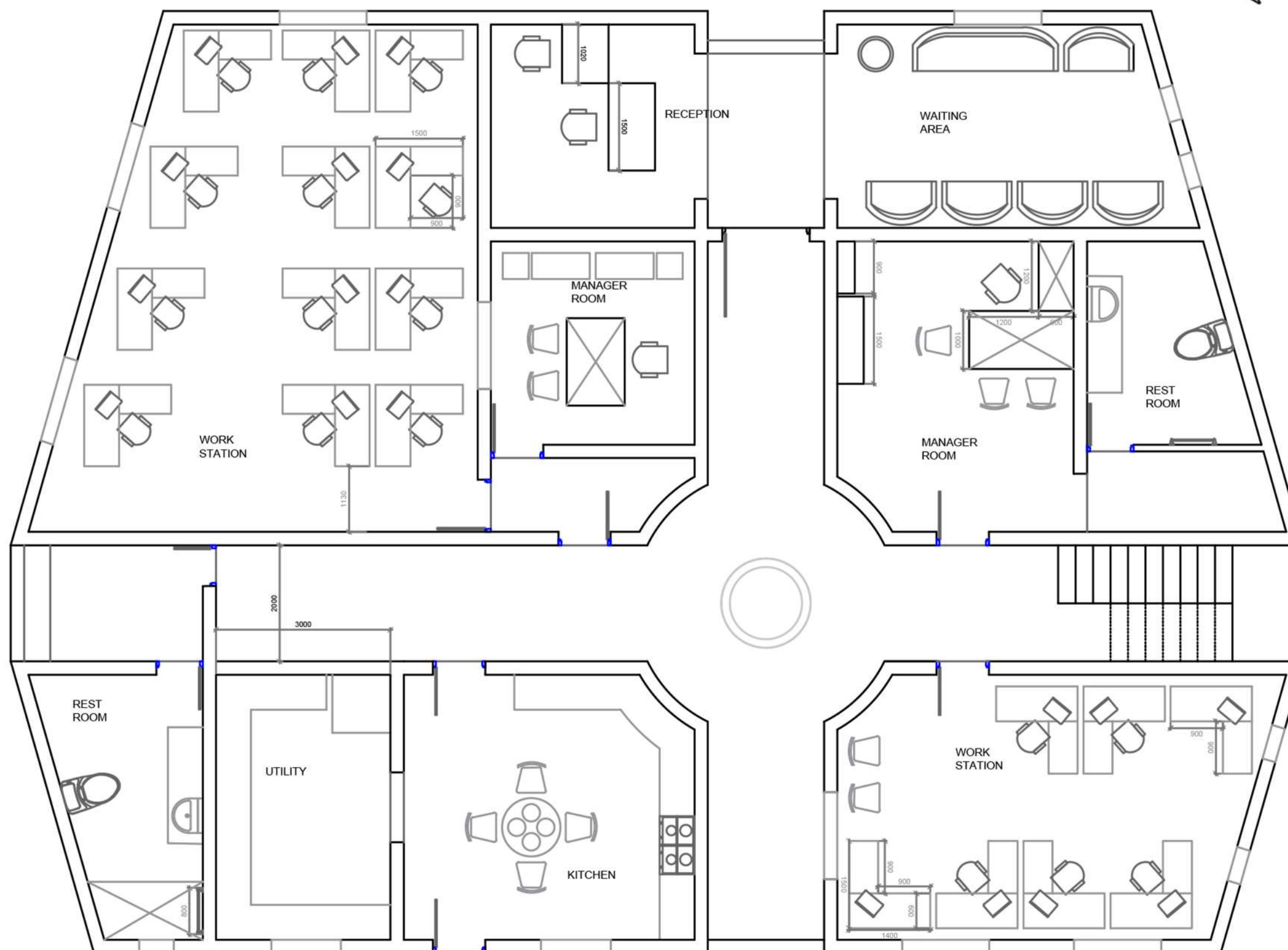
PLAN GROUND FLOOR
