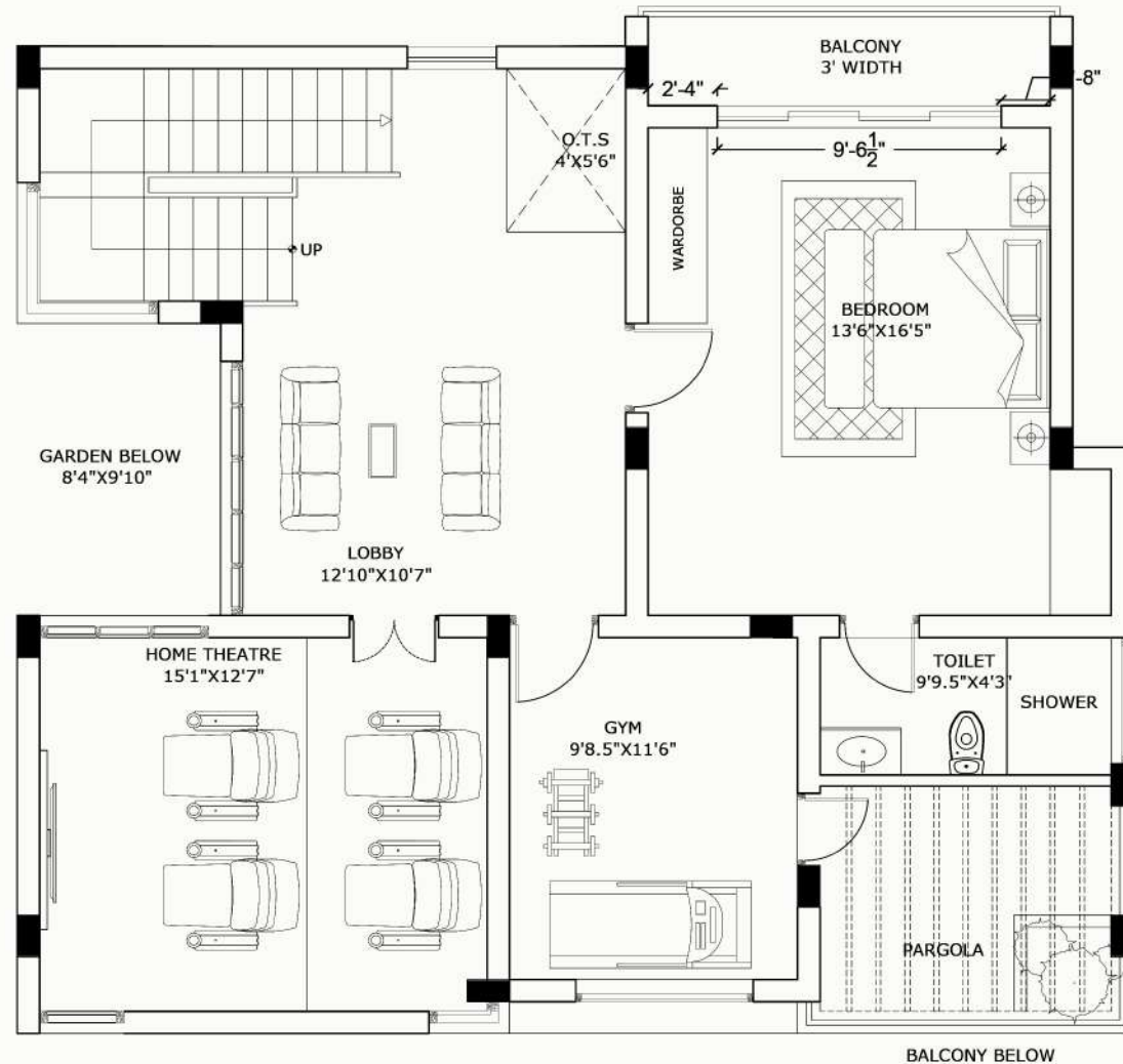
SECOND FLOOR -1054SQ. FT.
