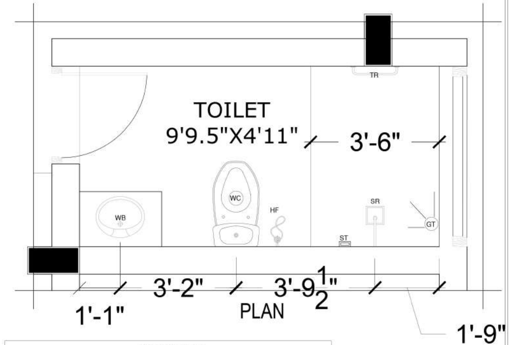
FIRST FLOOR TOILET 1
