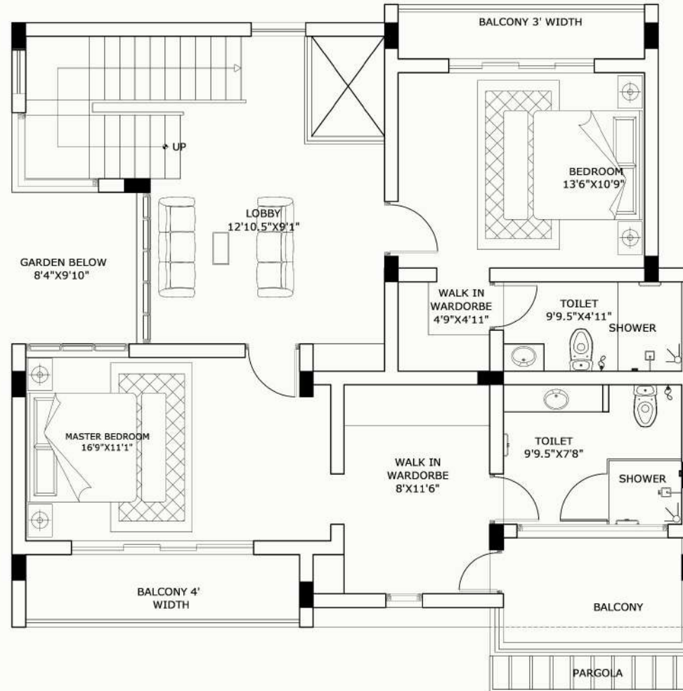
FIRST FLOOR - 1095 SQ. FT.
