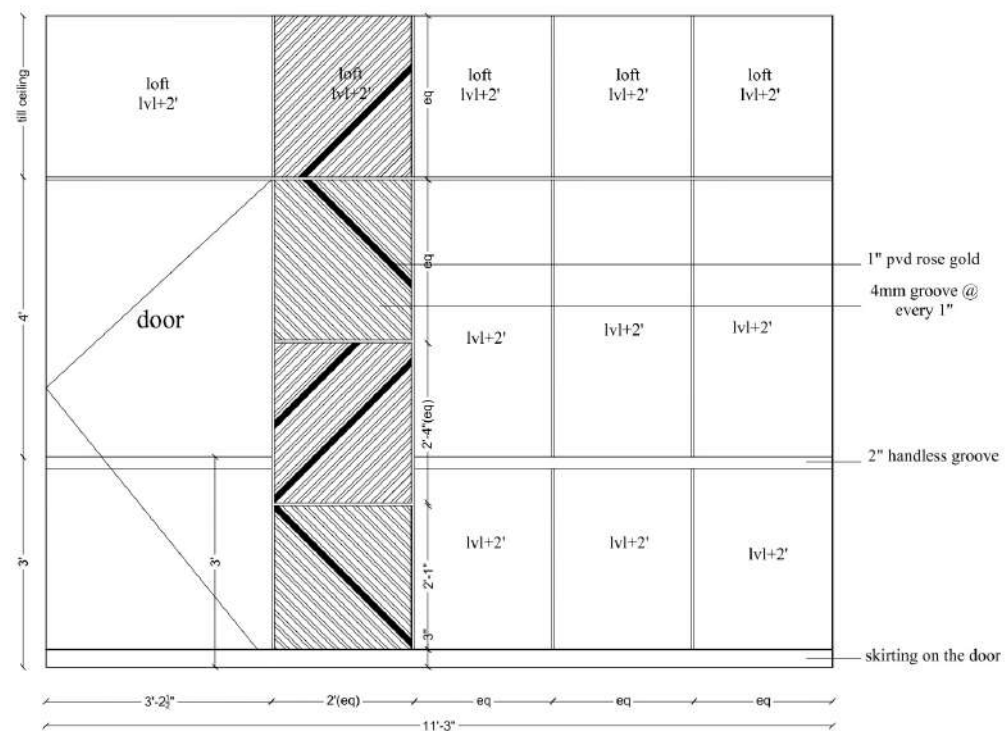
Dining elevation
