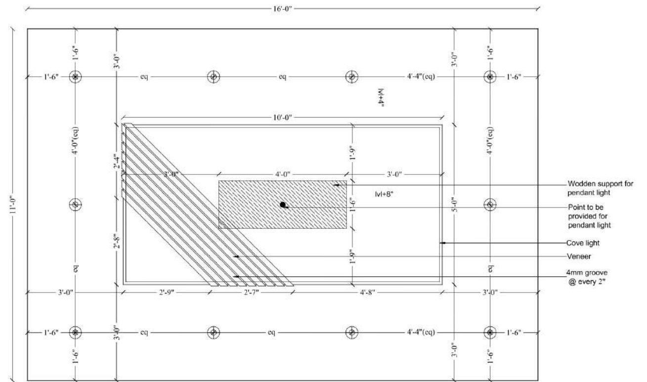
Ceiling plan
