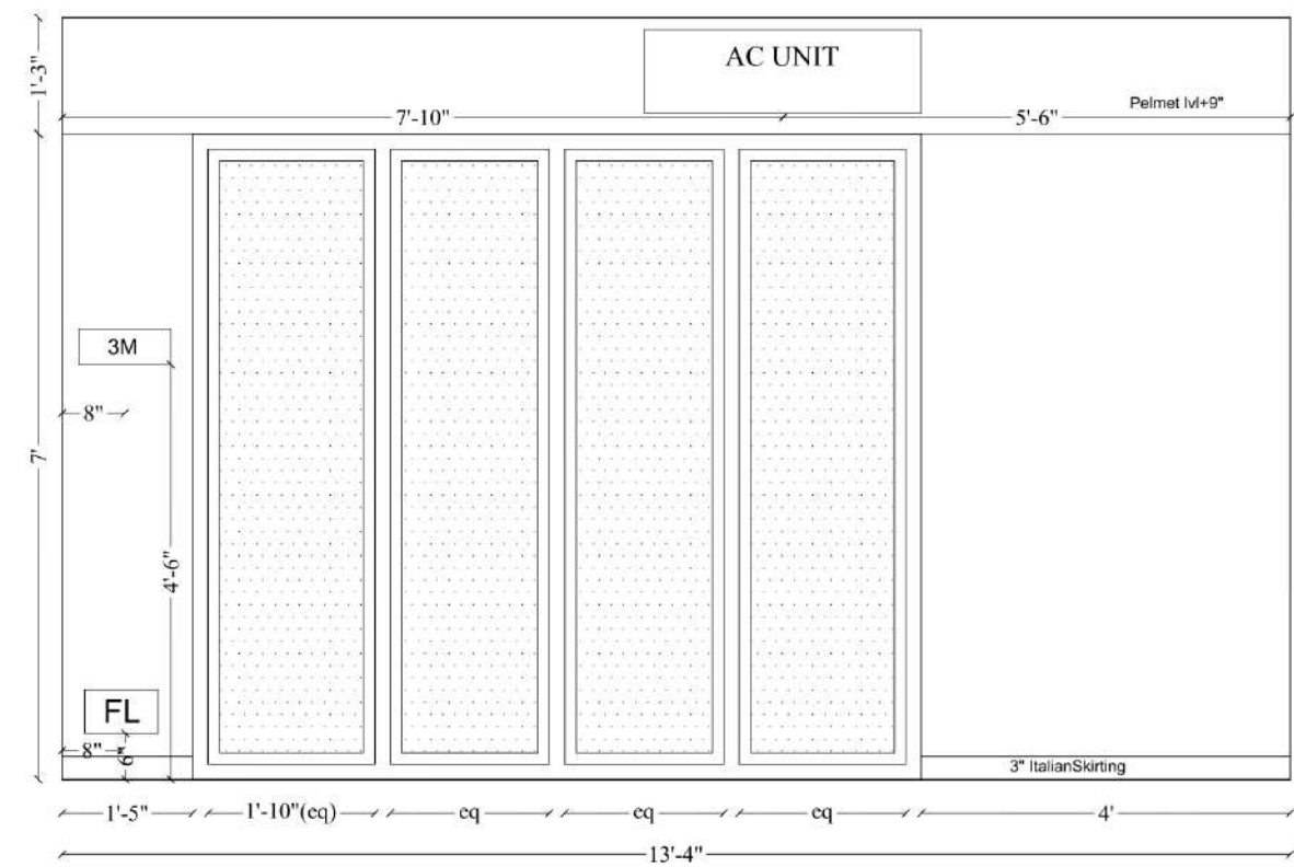
Elevation C
