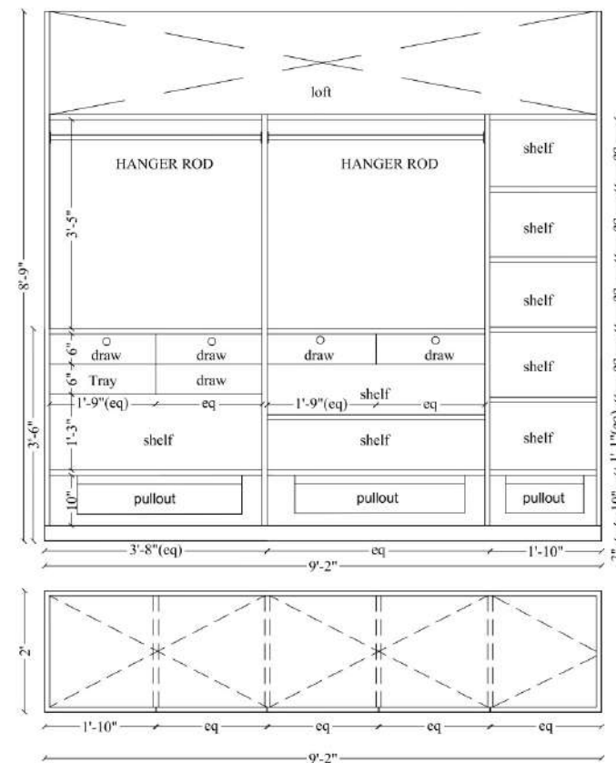
Wardrobe interior
