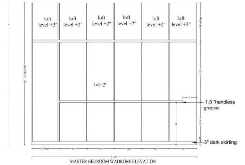
Elevation-C
