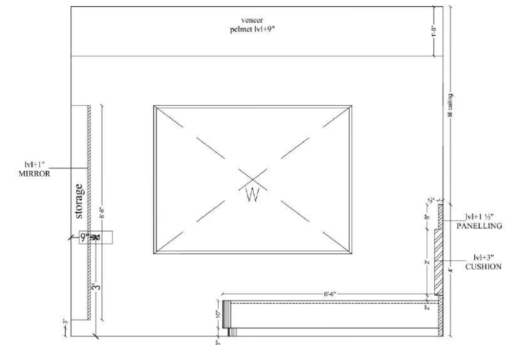
Elevation-D
