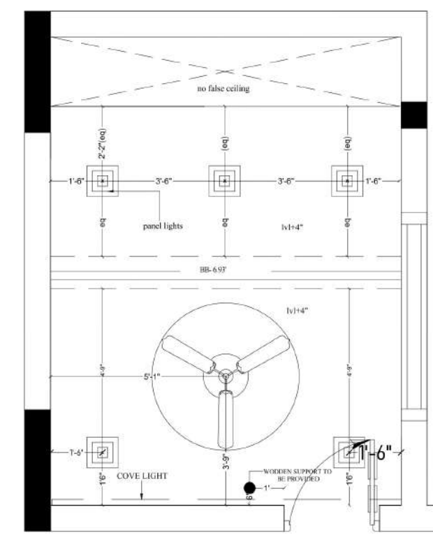
Ceiling plan
