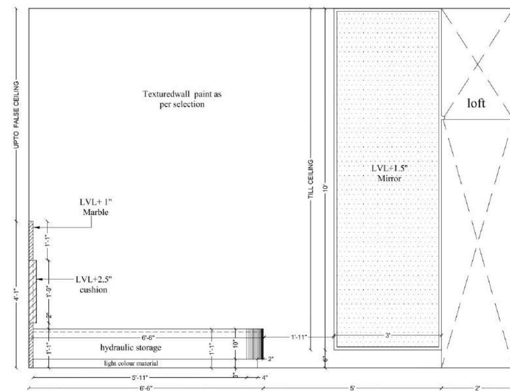
Elevation-D
