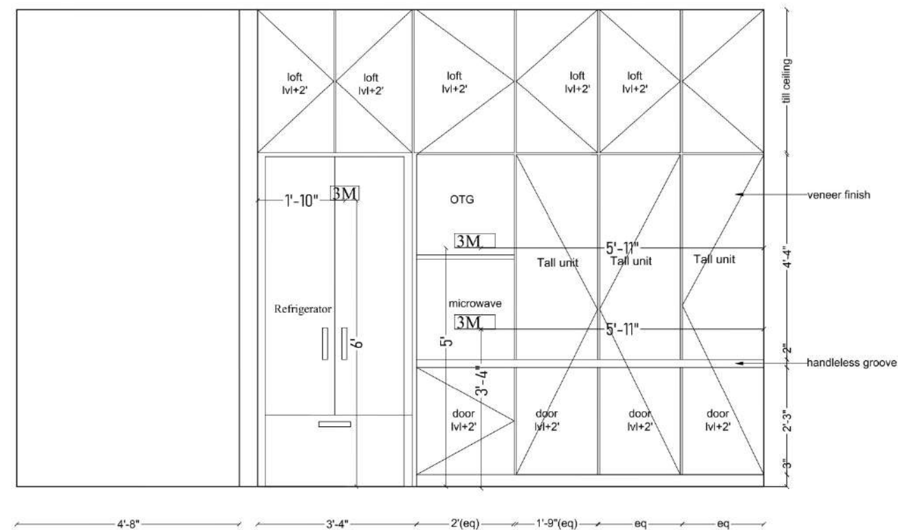
Elevation-D
