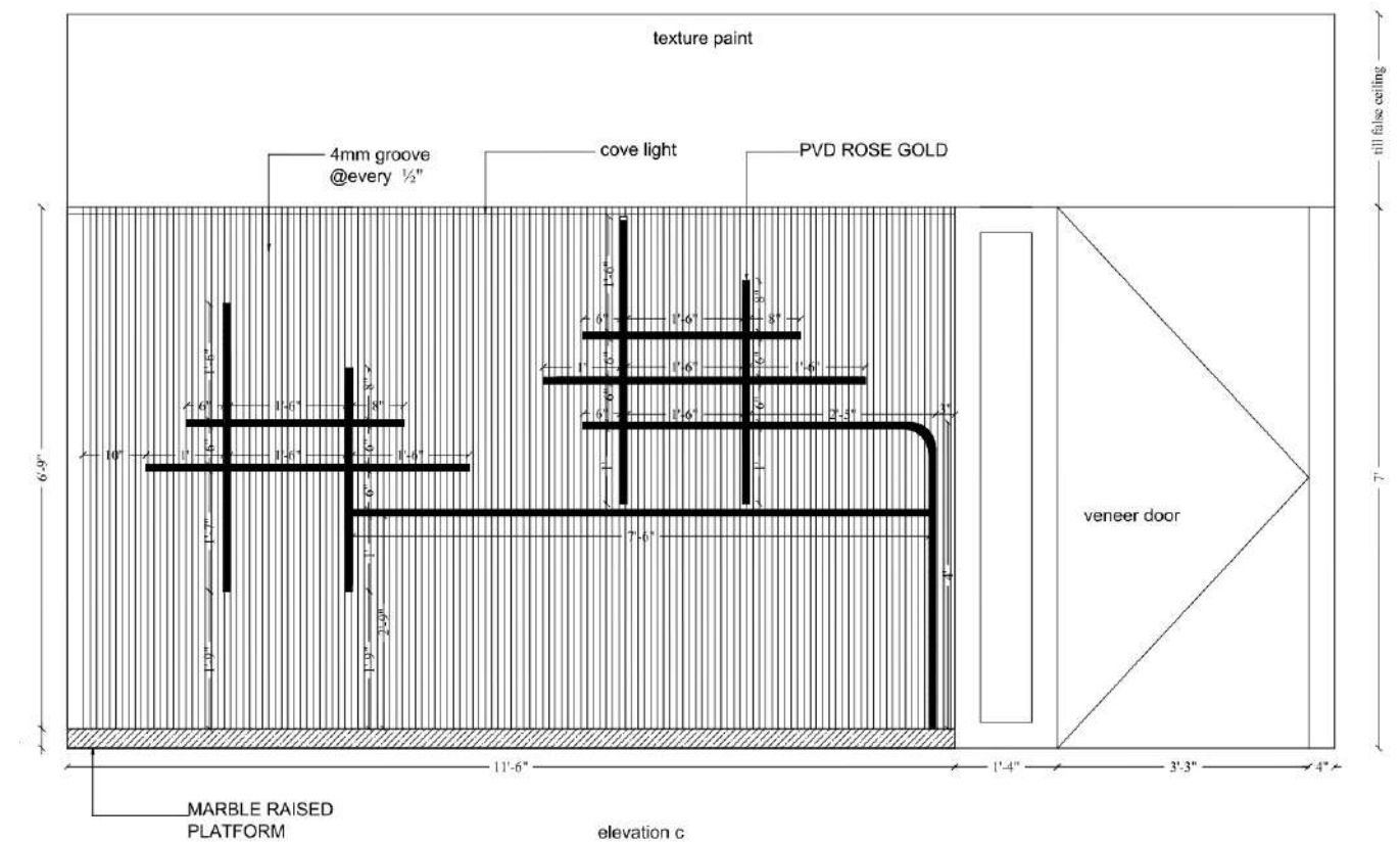
Elevation C
