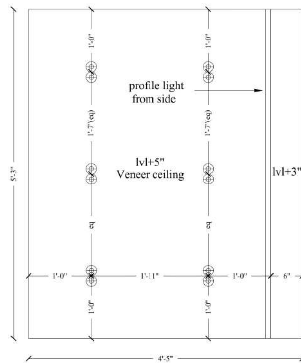
Ceiling plan
