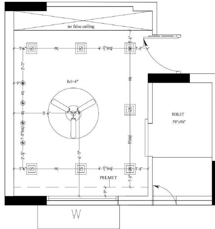
Ceiling plan
