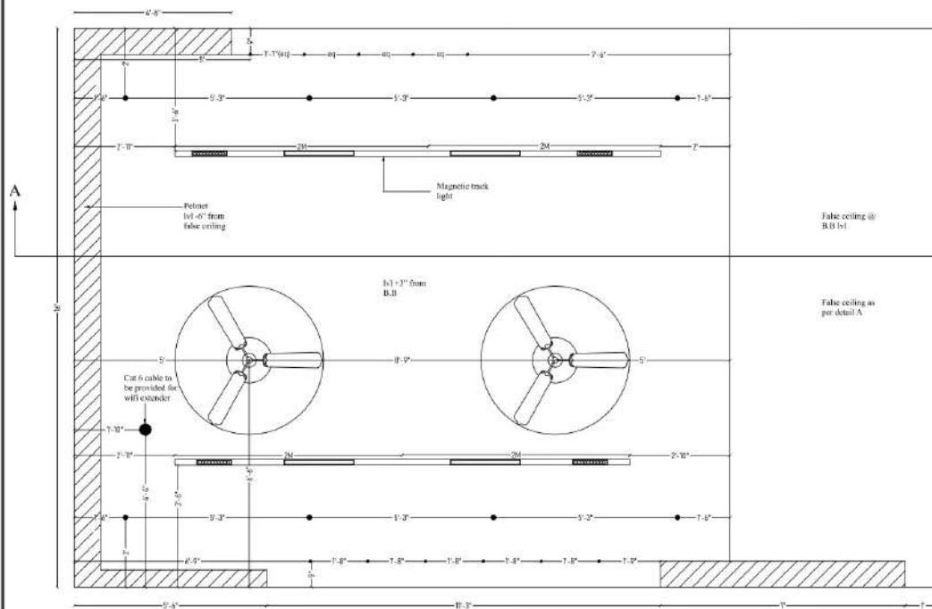
Ceiling plan
