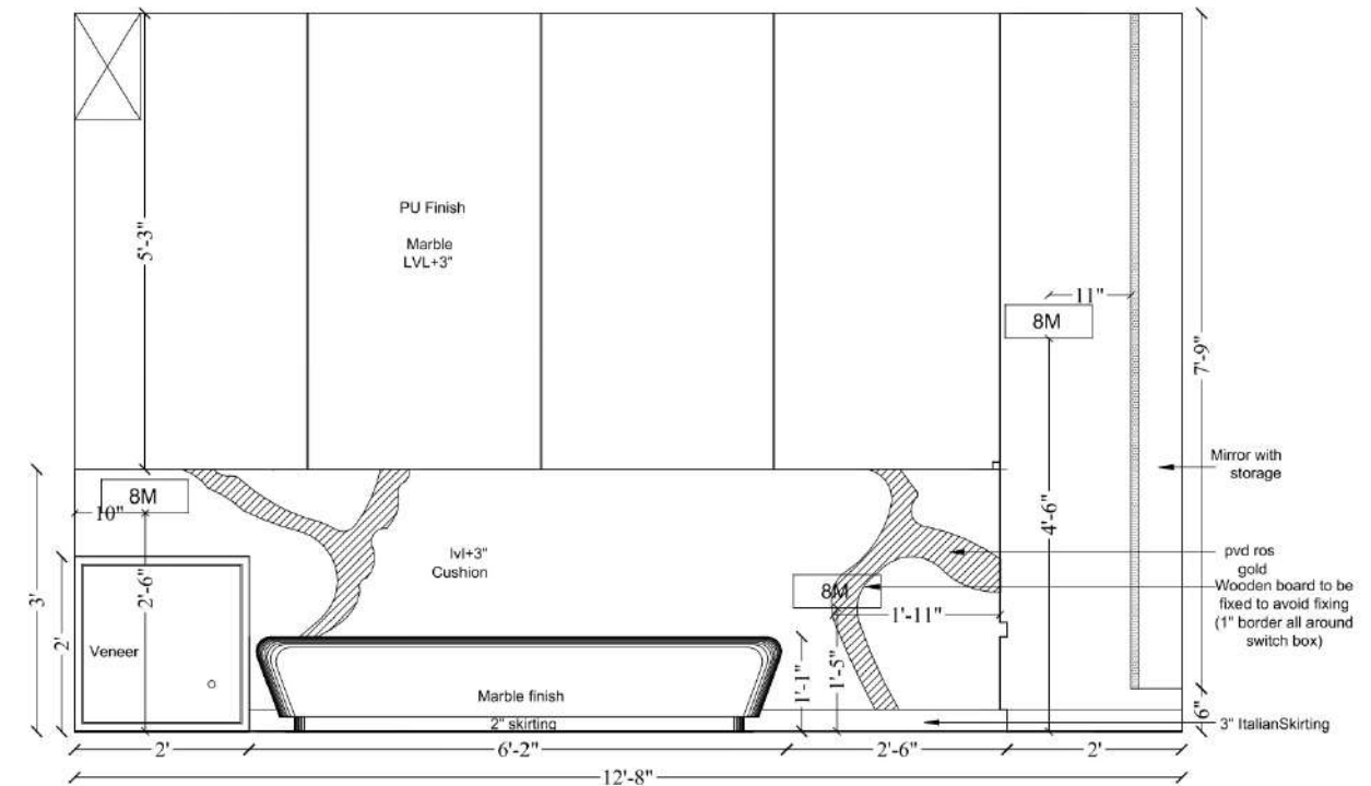
Elevation D
