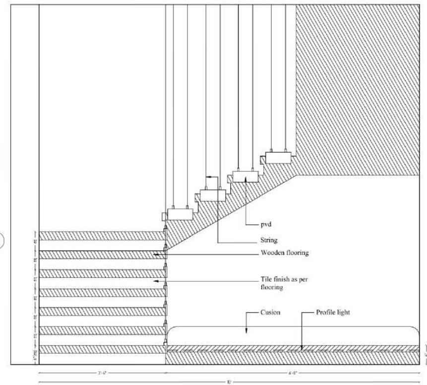
Staircase detail
