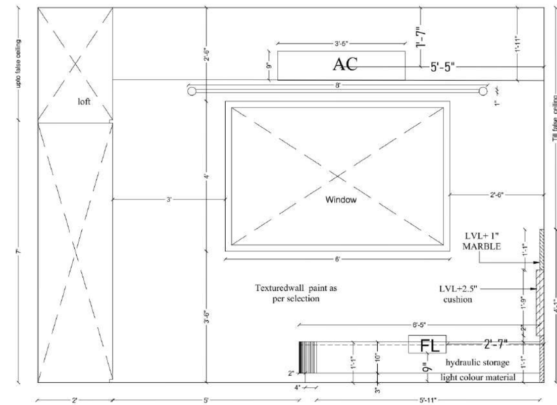
Elevation-B
