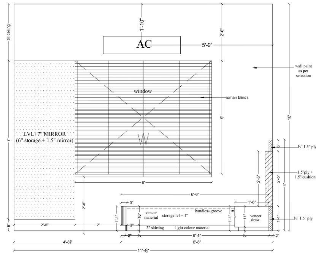
Elevation-D
