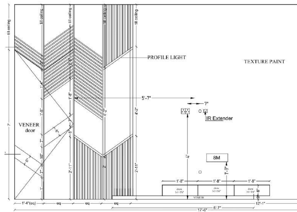
Tv wall
