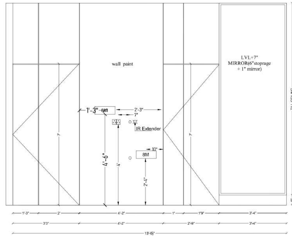
Elevation-C
