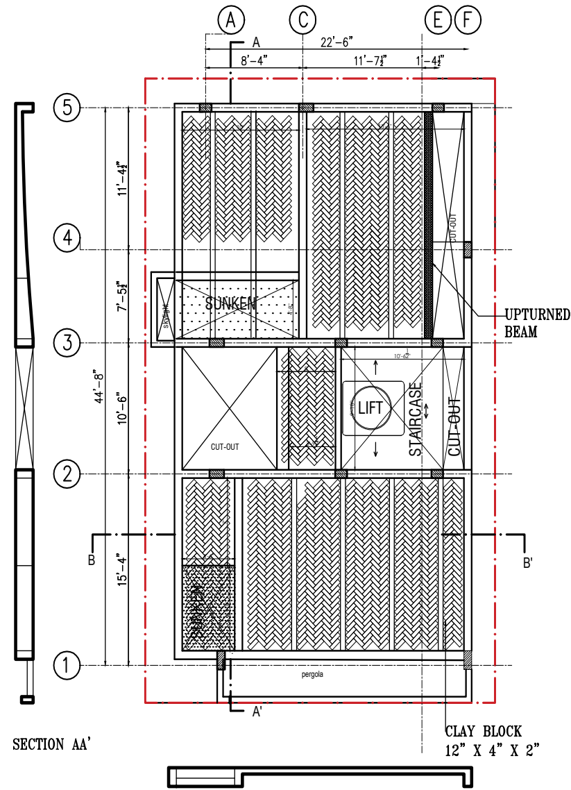
FIRST FLOOR BEAM LAYOUT
