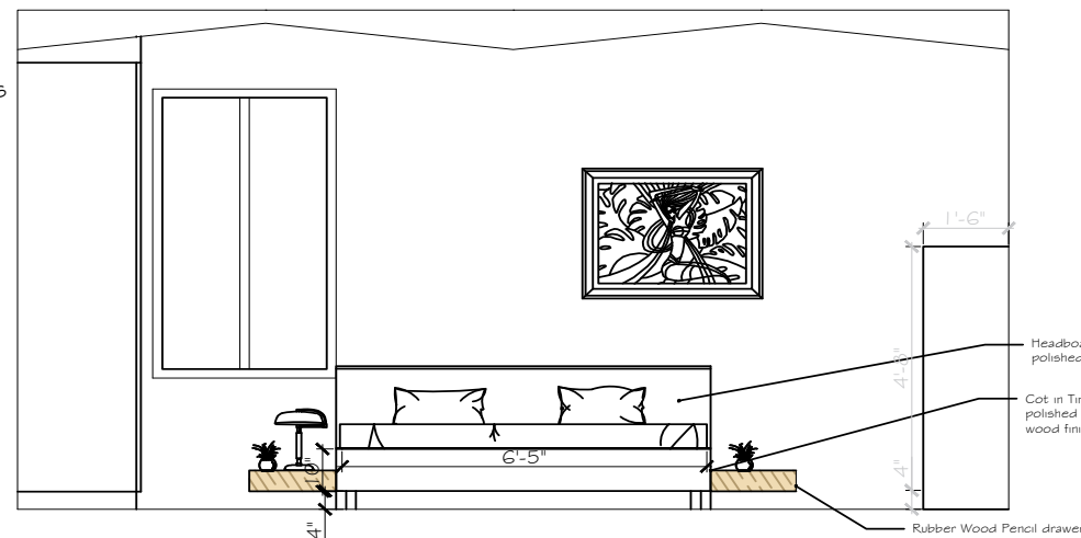
BED ELEVATION
