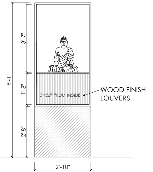
ELEVATION -SIDE A FROM STAIRCASE SIDE
