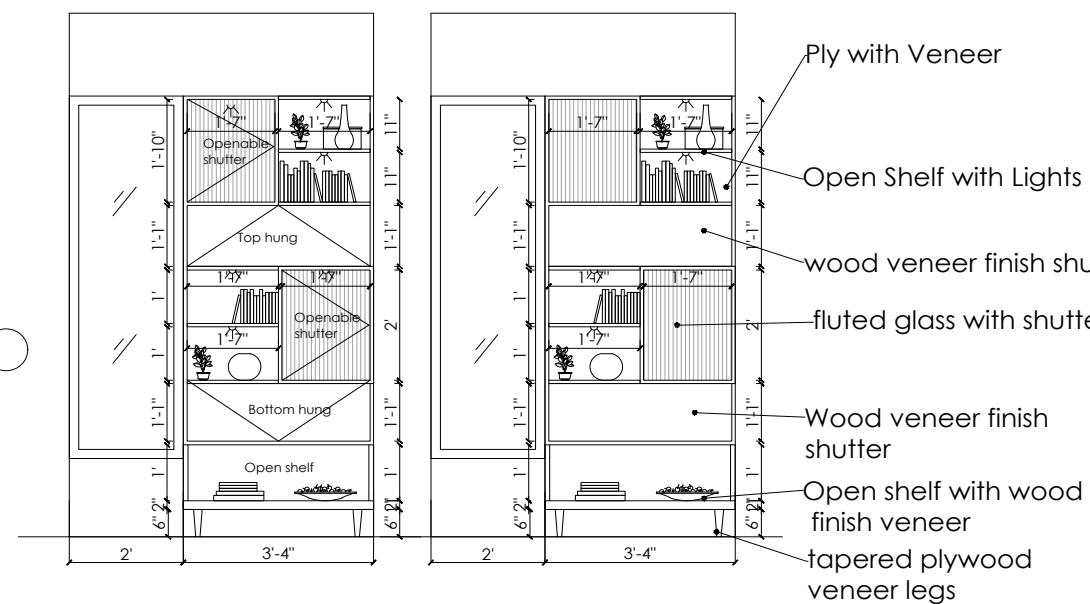
ELEVATION - book shelf
