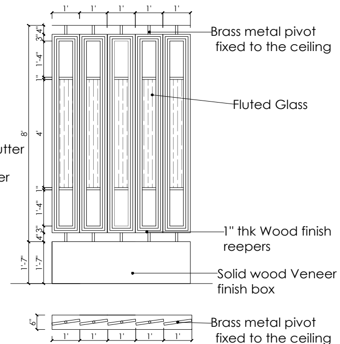
PARTITION ELEVATION
