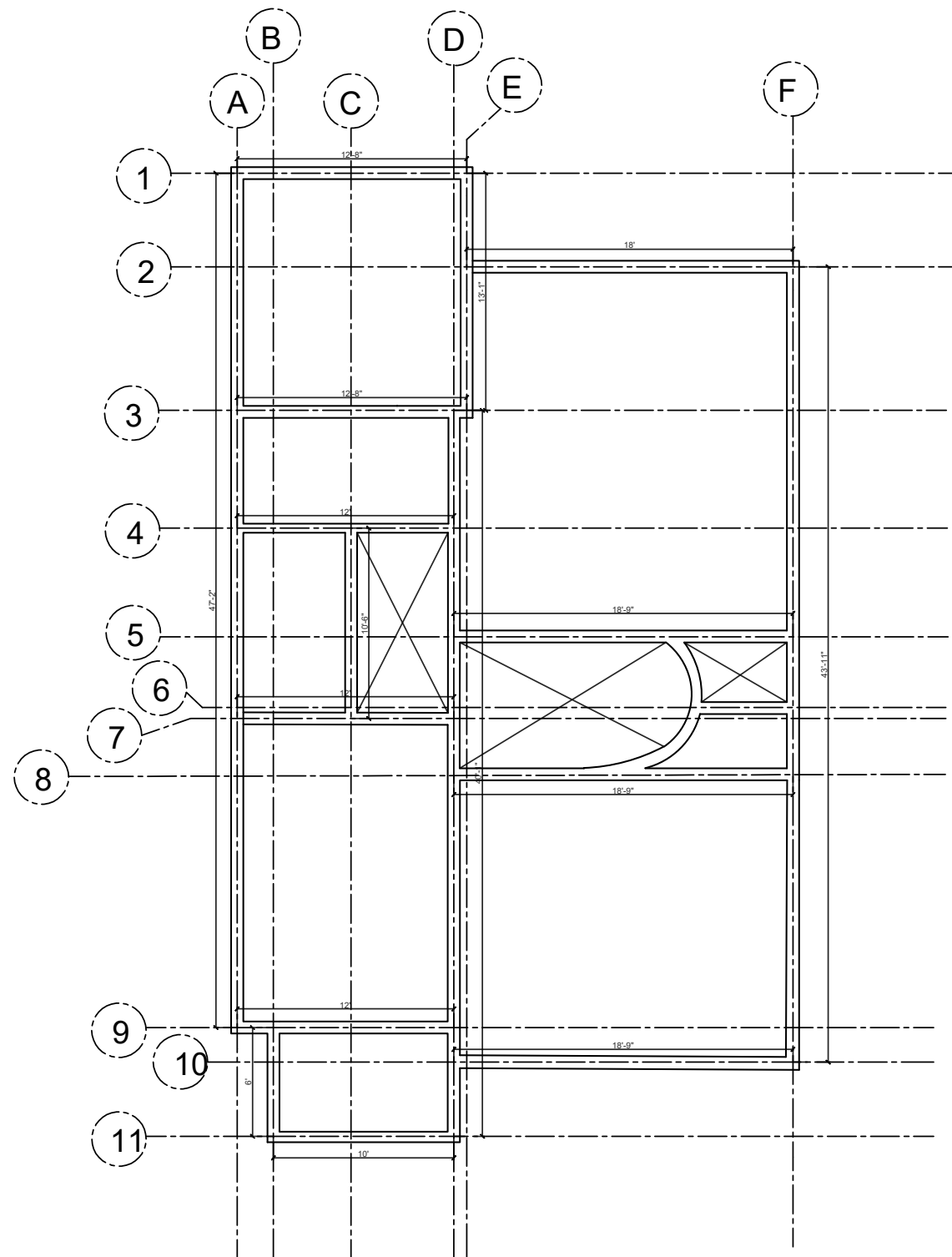
GF - ROOF BEAM LAYOUT
