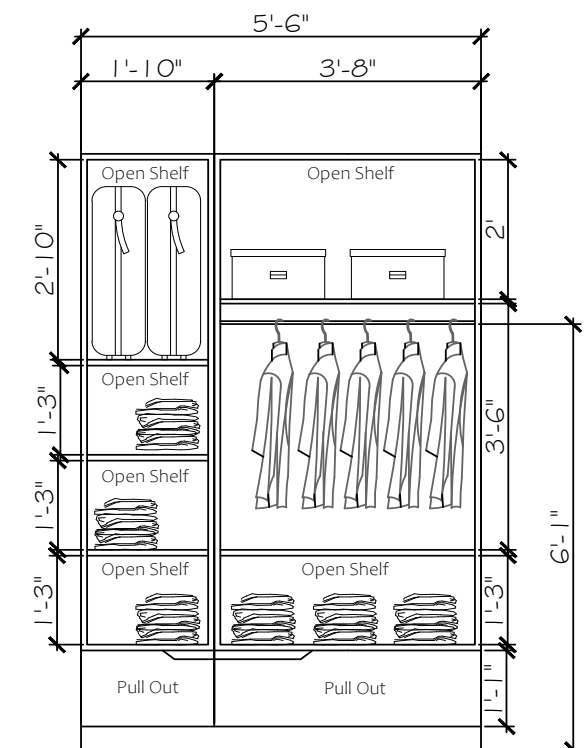
WARDROBE INTERIORS
