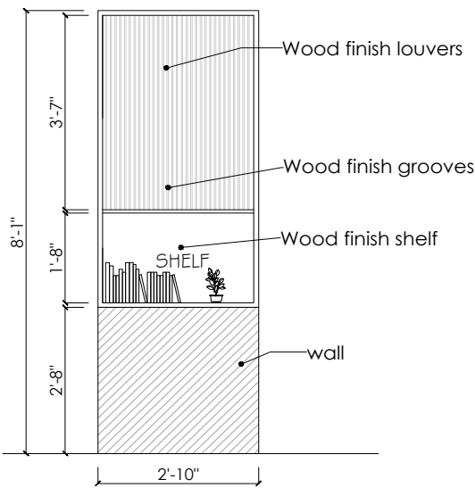
ELEVATION -SIDE B FROM DINING SIDE
