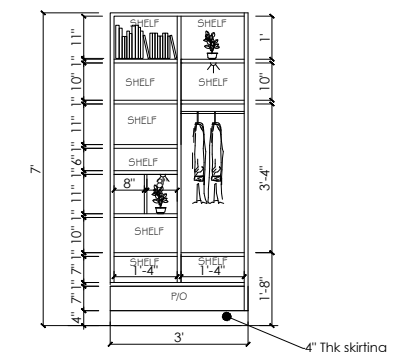
STORAGE
