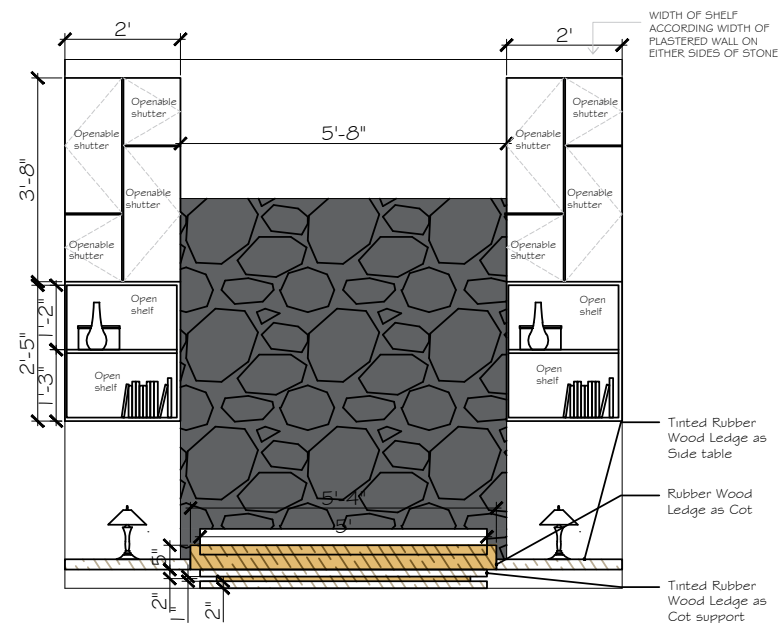
BED ELEVATION
