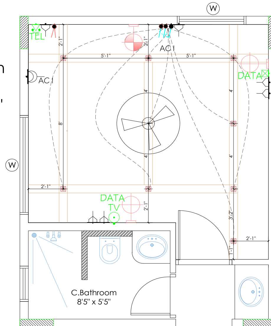
ELECTRICAL PLAN
