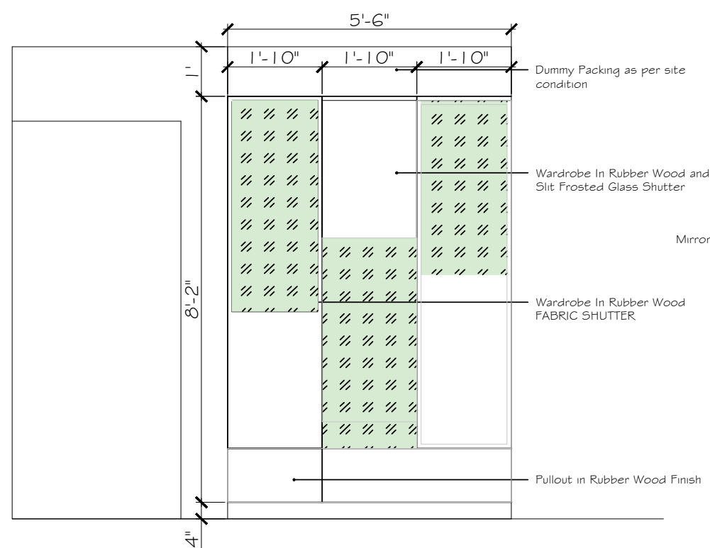
WARDROBE ELEVATION
