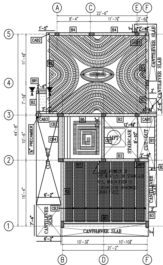
GROUND FLOOR BEAM LAYOUT
