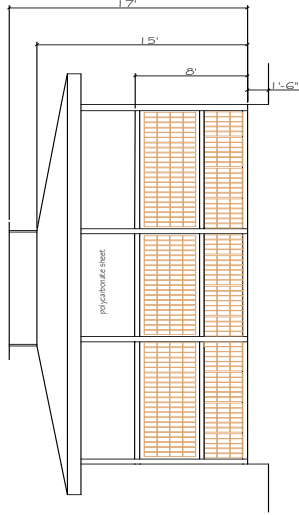
ELEVATION D
