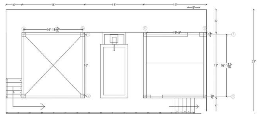
COLUMN LAYOUT
