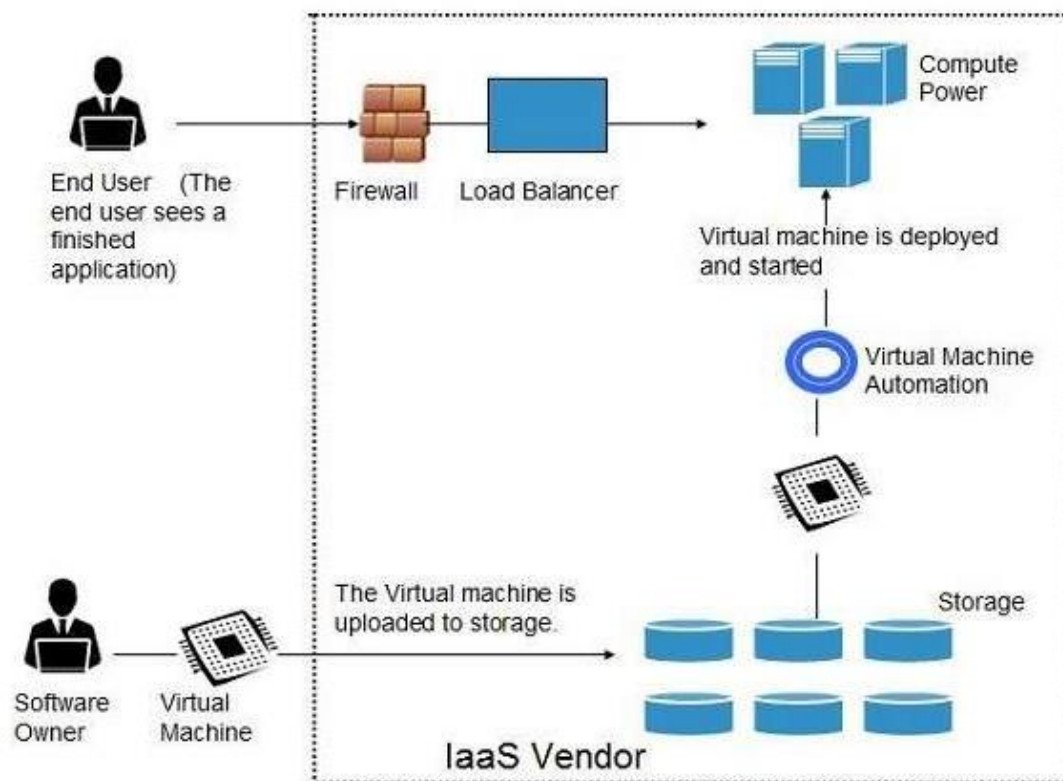
Fig 2.4.1 Infrastructure As a Service
