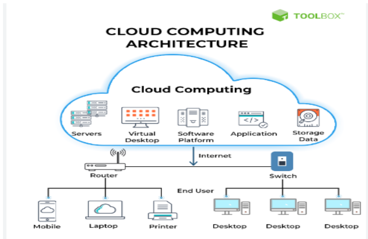
Fig 2.1 Cloud Computing
