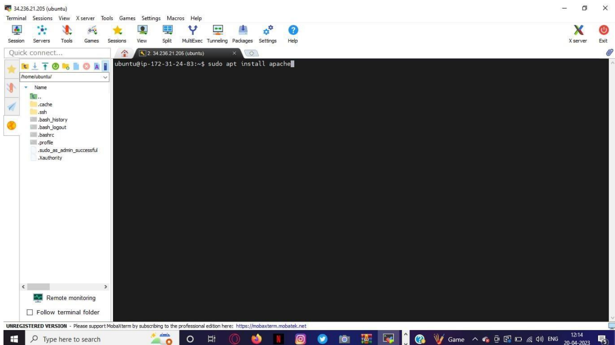
Fig 7.6: CD/TMP
