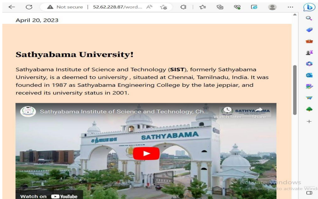
Fig 8.2: OUTPUT 2
