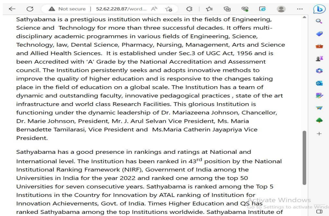
Fig 8.3
