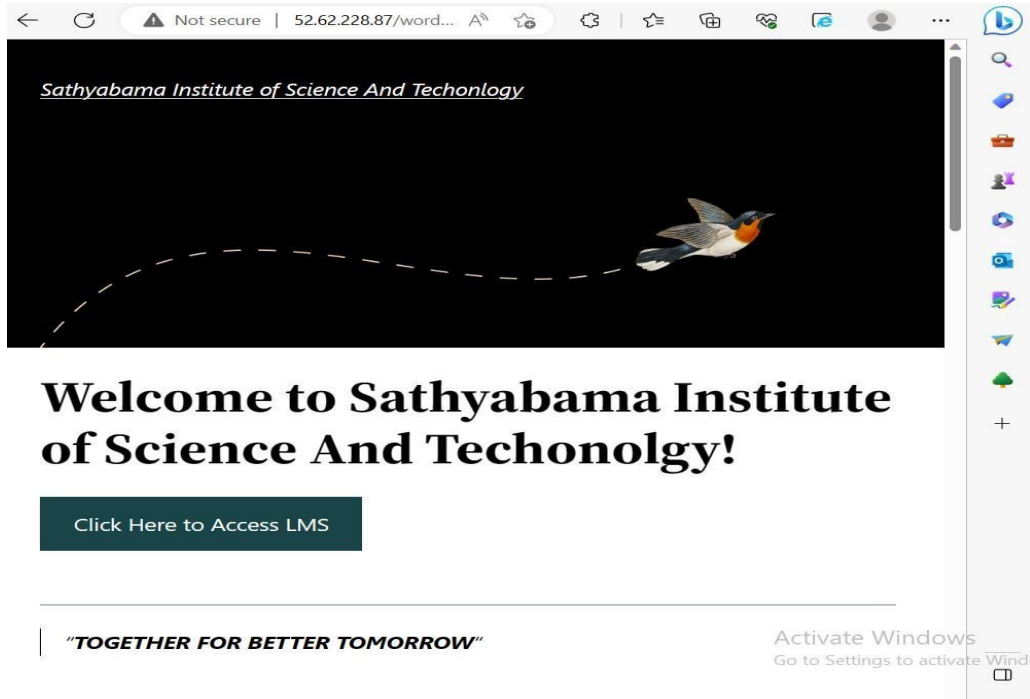
Fig 8.1: OUTPUT 1
