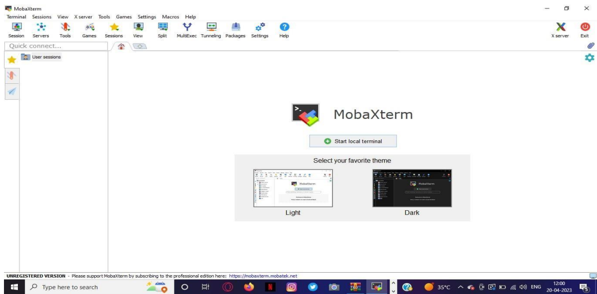
Fig 6.3 : INSTALLING MOBAXTERM
