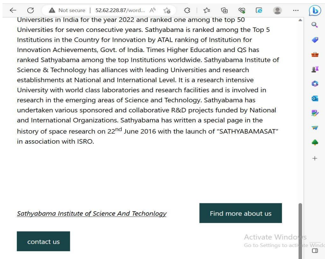
Fig 8.4
