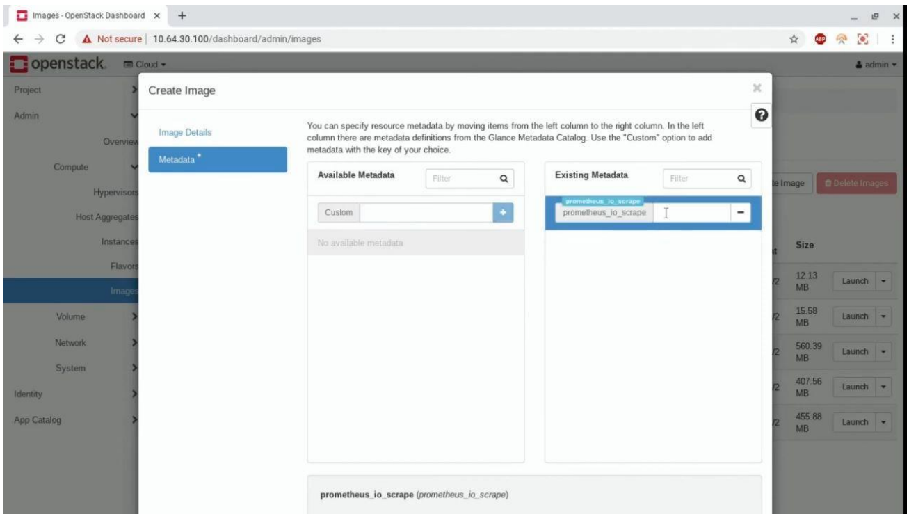
FIG.3.3.7 Create Image
