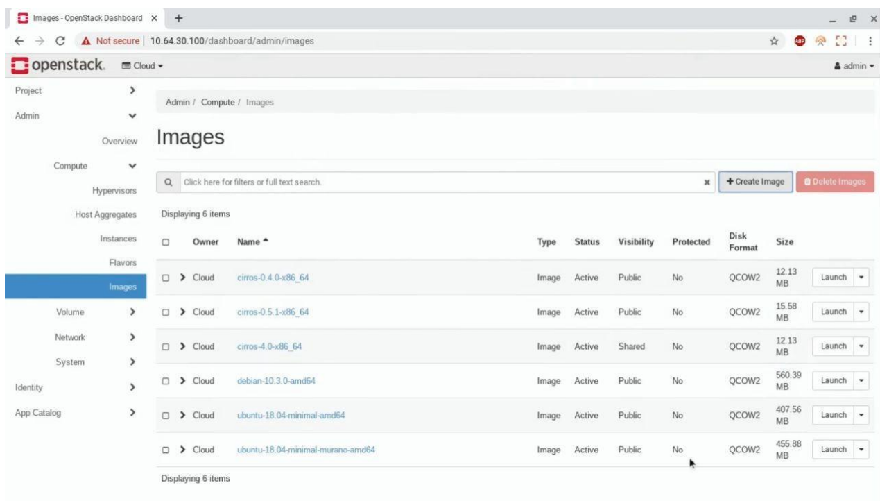
FIG.3.3.4 Images
