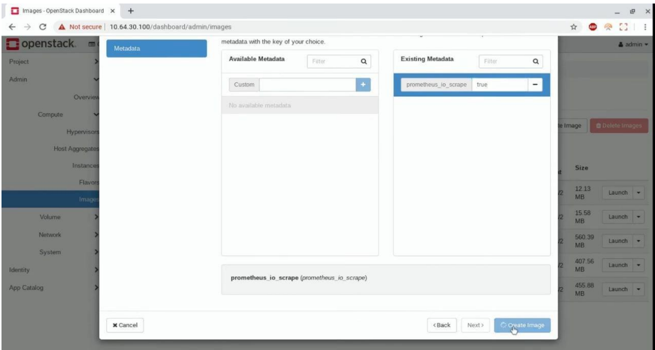
FIG.3.3.8 Metadata
