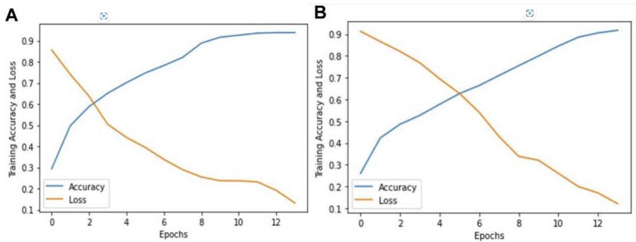
Fig.5.1. ResNet 50 vs Inception v3
