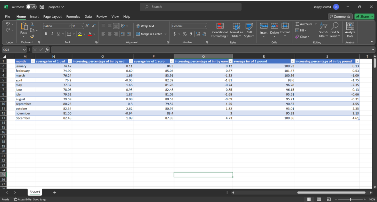
FIGURE 5.3 : DATASET 1
