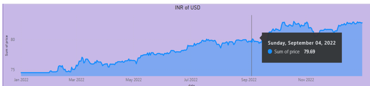
FIGURE 6.4 : USD ANALYSIS
