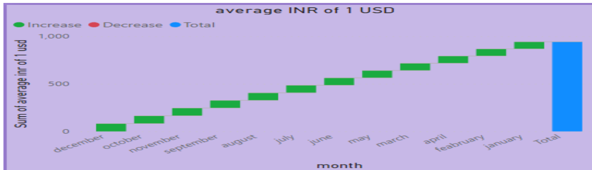
FIGURE 6.5 : AVERAGE USD
