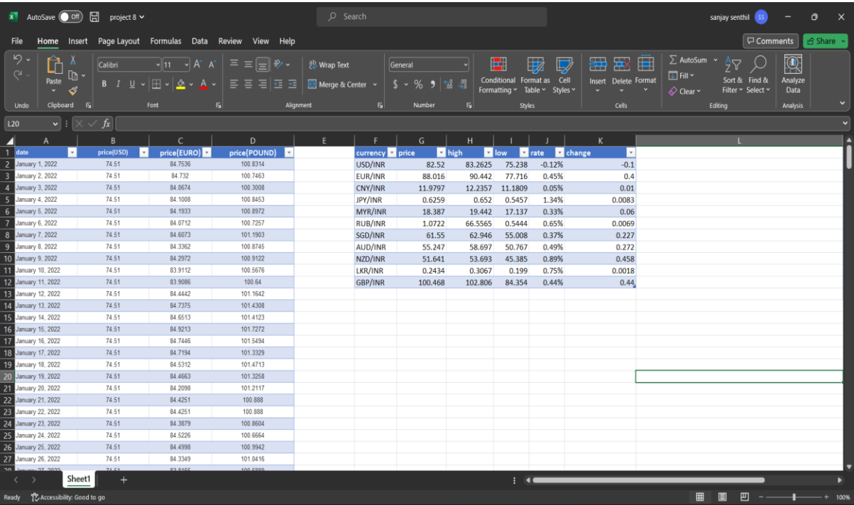
FIGURE 5.4 : DATASET 2
