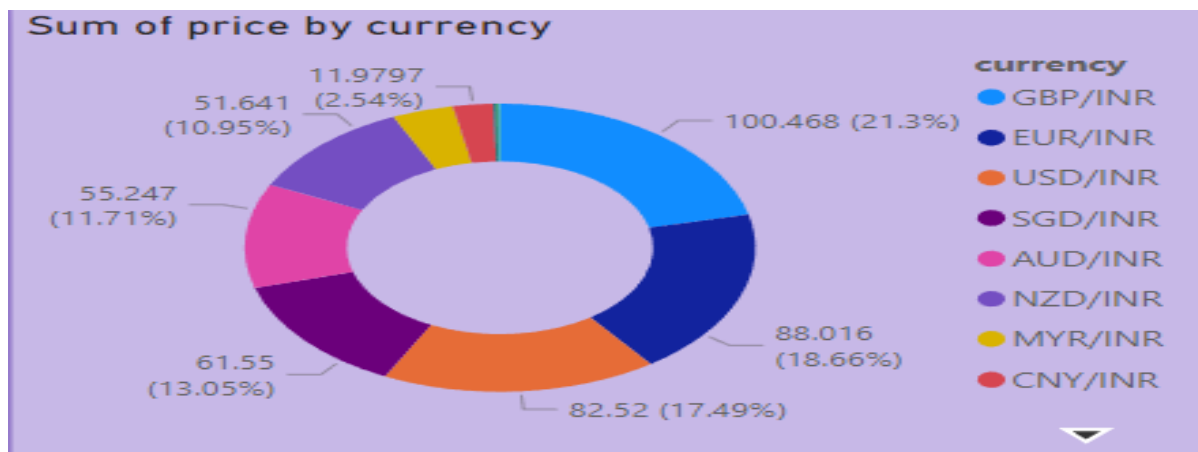
FIGURE 6.13 : CURRENT PRICE
