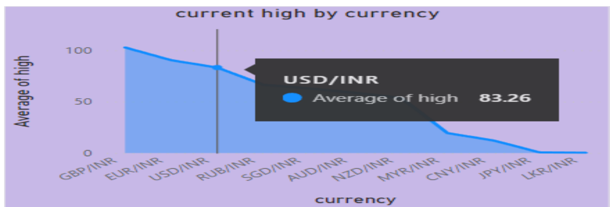
FIGURE 6.15 : CURRENT HIGH
