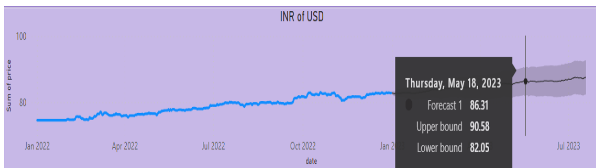
FIGURE 6.1 : PREDICTION TABLE
