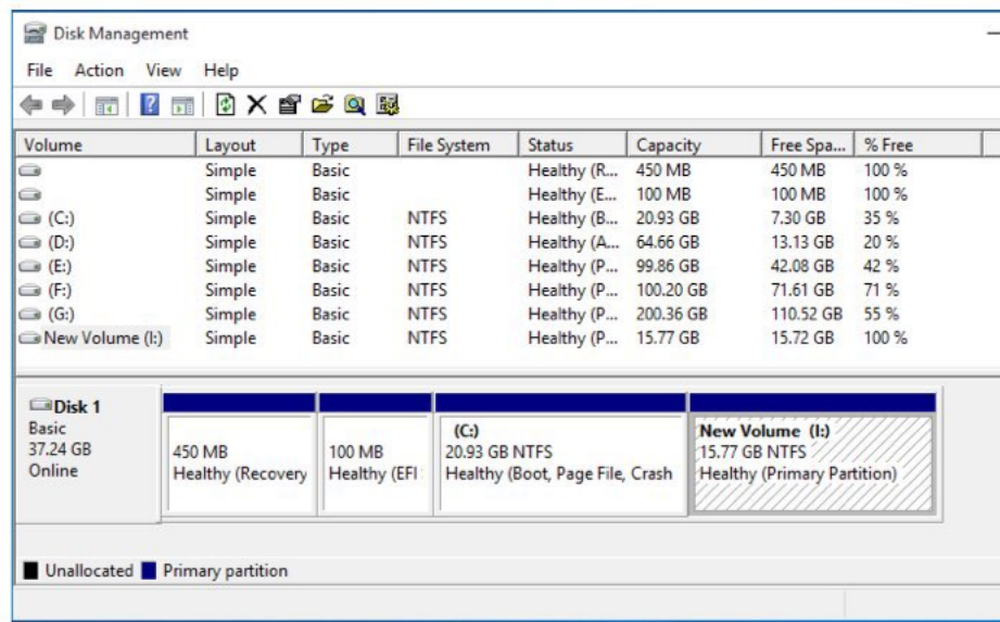
Fig 4.4 Disk management
