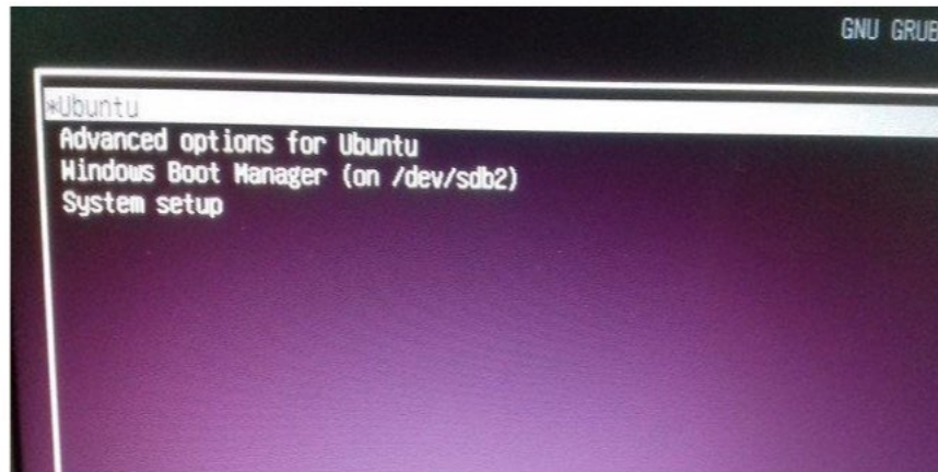
Fig 4.8 GRUB Menu
