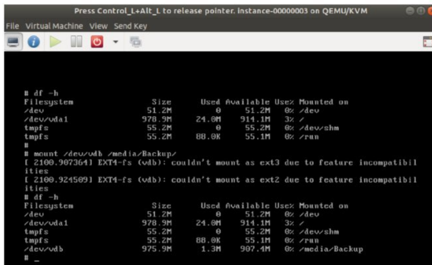
Fig:4.26 Mounting volume
