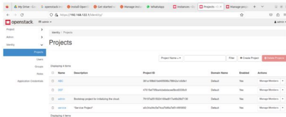
Fig 5.1 create project
