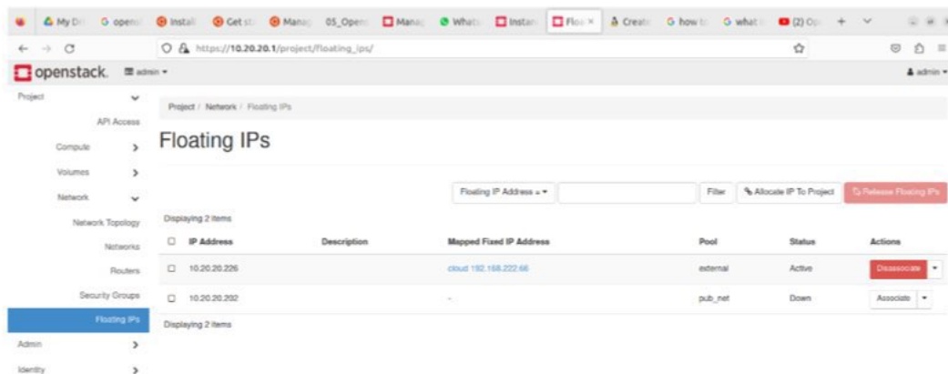
Fig 5.8 Floating Ips
