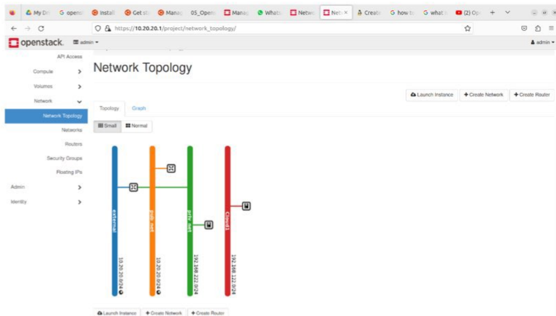
Fig 5.5 Network topology
