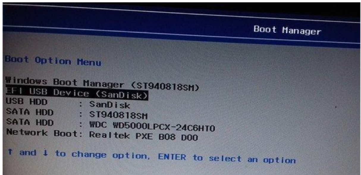
Fig 4.5 Boot manager
