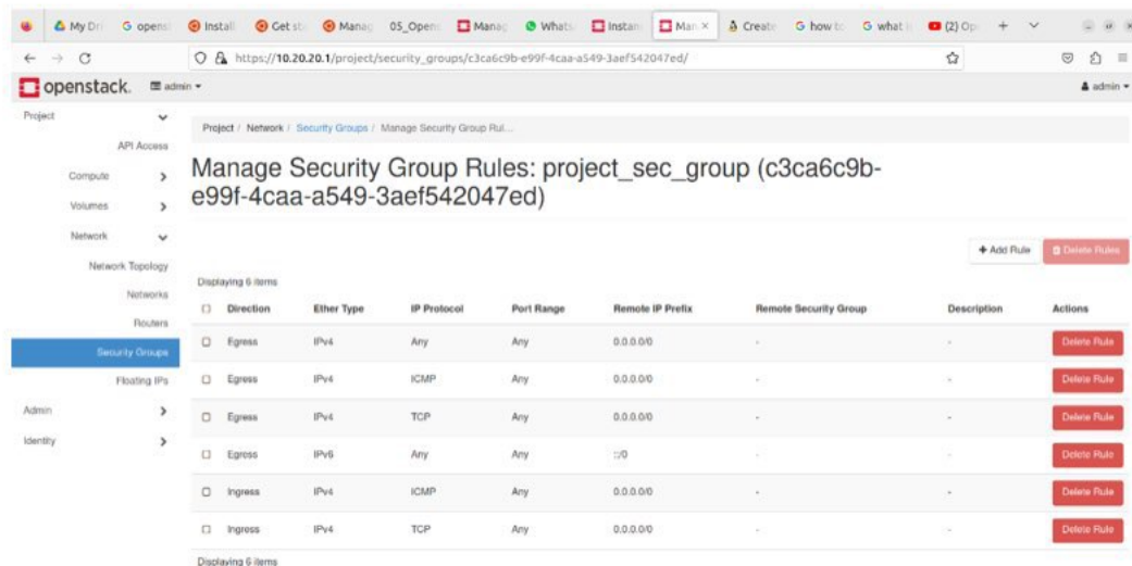
Fig 5.7 Manage rules
