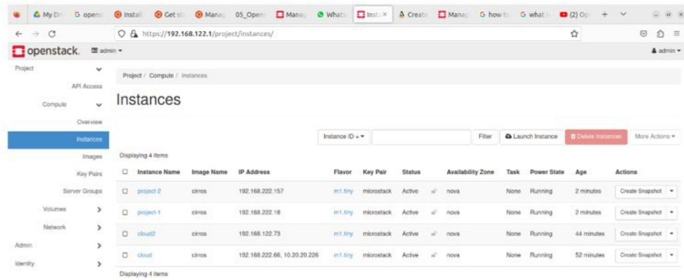
Fig 5.9 Create instance
