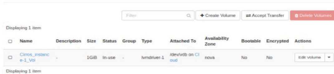
Fig 4.25 Volume Creation
