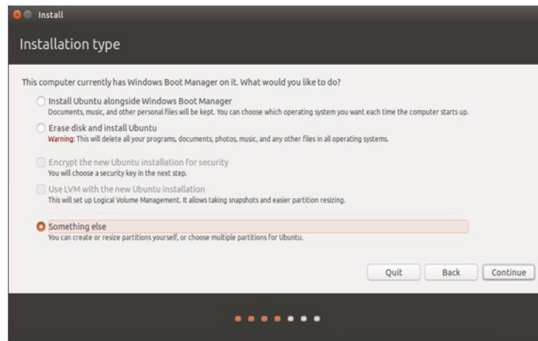
Fig 4.6 Installation Type
