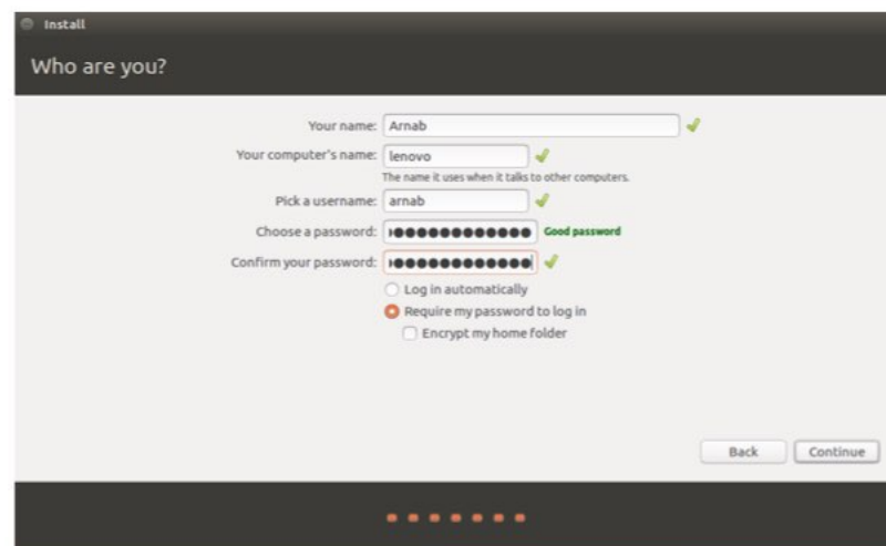
Fig 4.7 Setting Password
