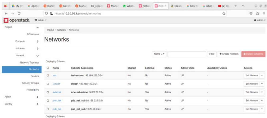
Fig 5.3 Create network
