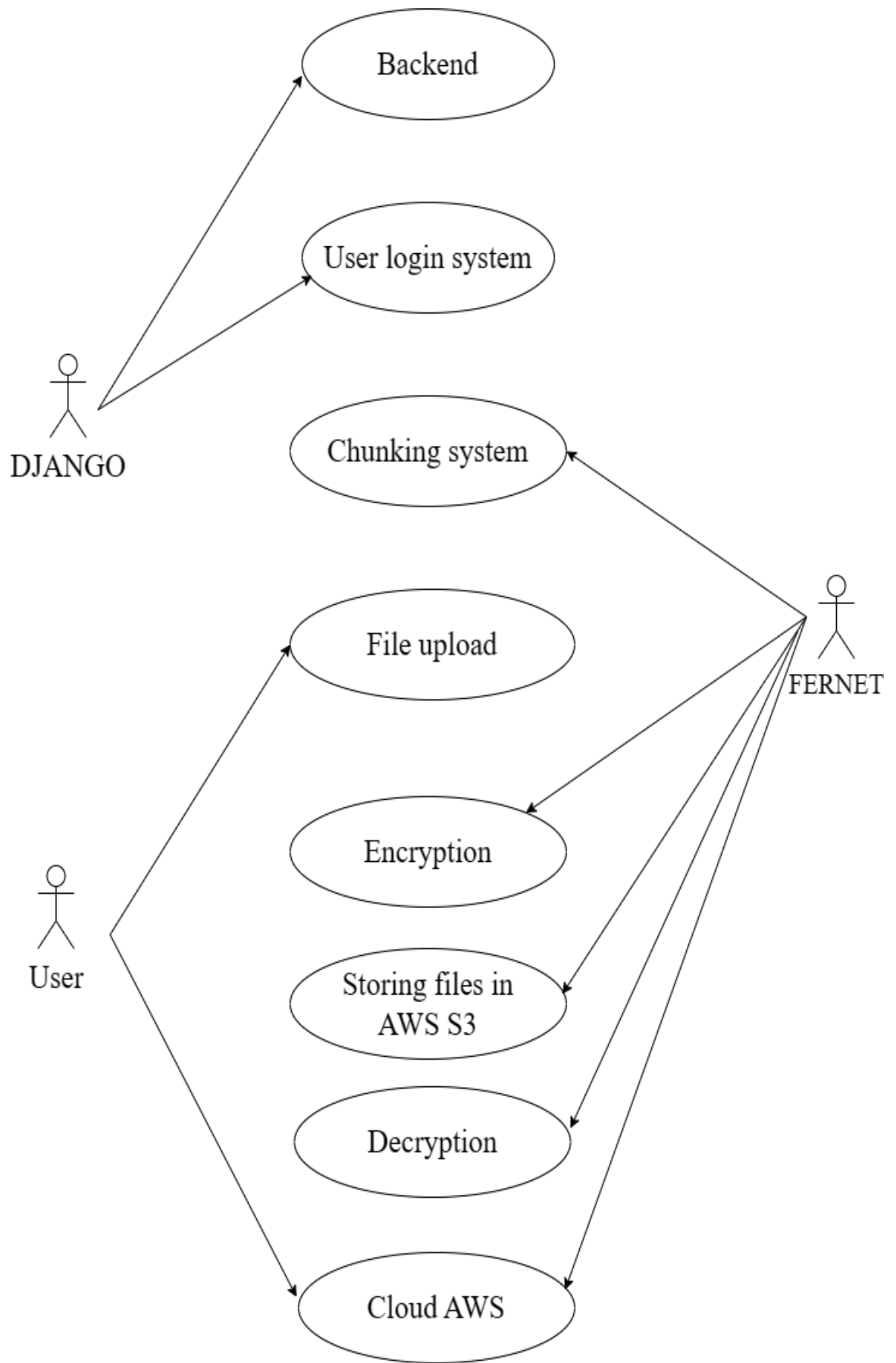
Fig 3.4 – Use-Case Diagram
