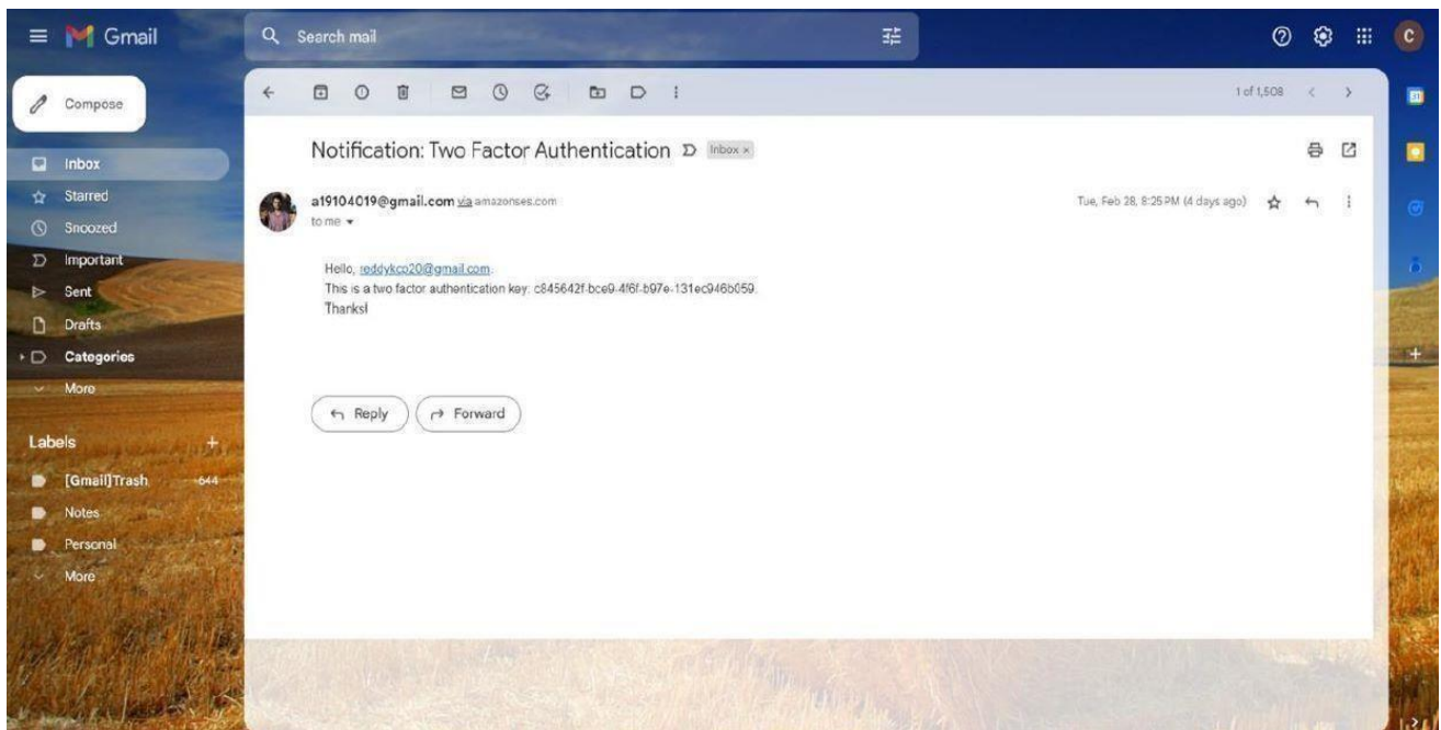
Fig 4.1 Screenshot 1
