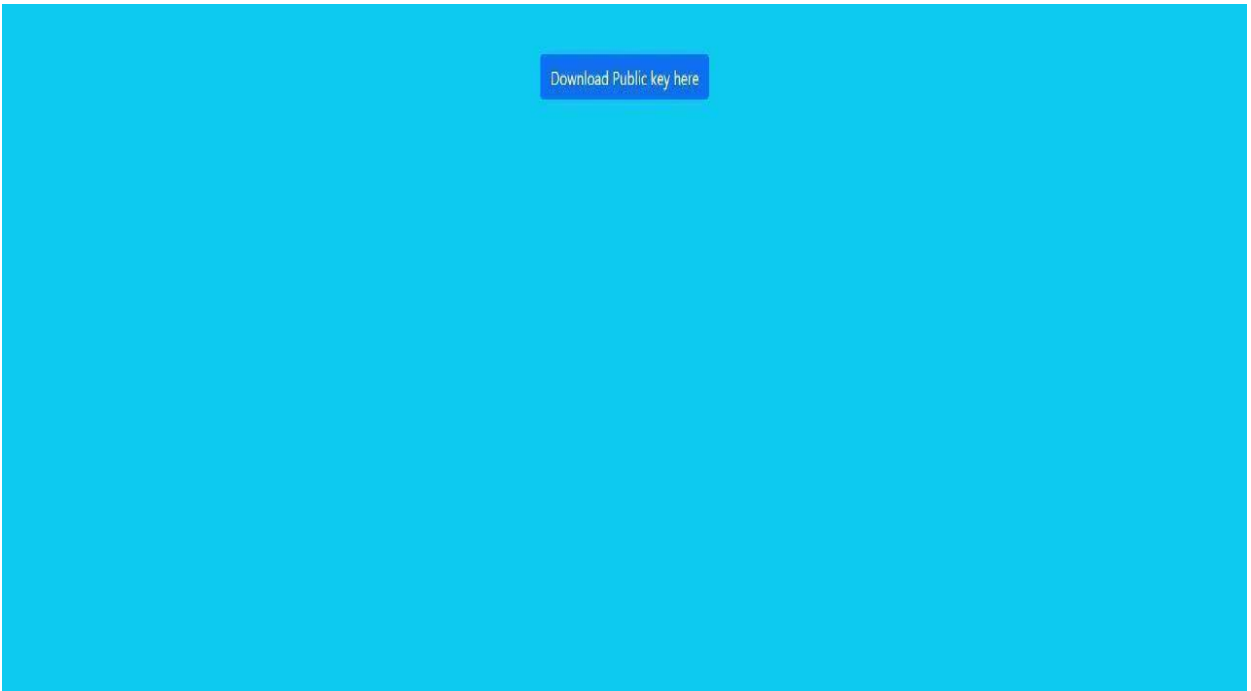
Fig 4.4 Screenshot 4
