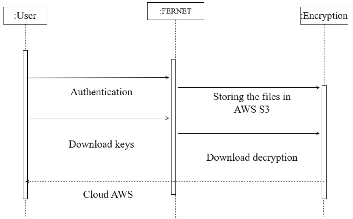
Fig 3.6 – Sequence Diagram
