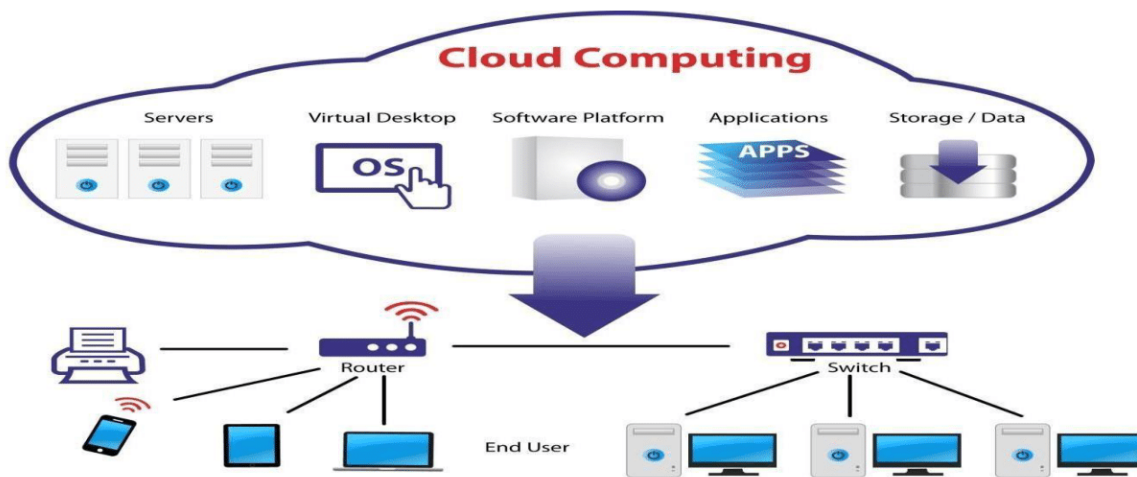
Fig 2.1 Cloud Computing
