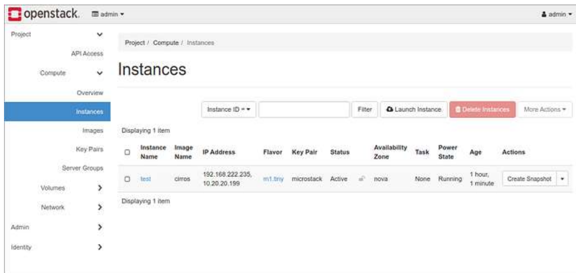
Fig 6.1: Created Instance
