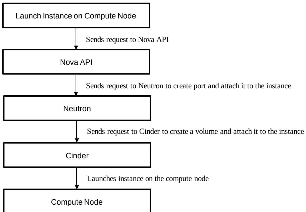
Fig. 5.7 Compute Node
