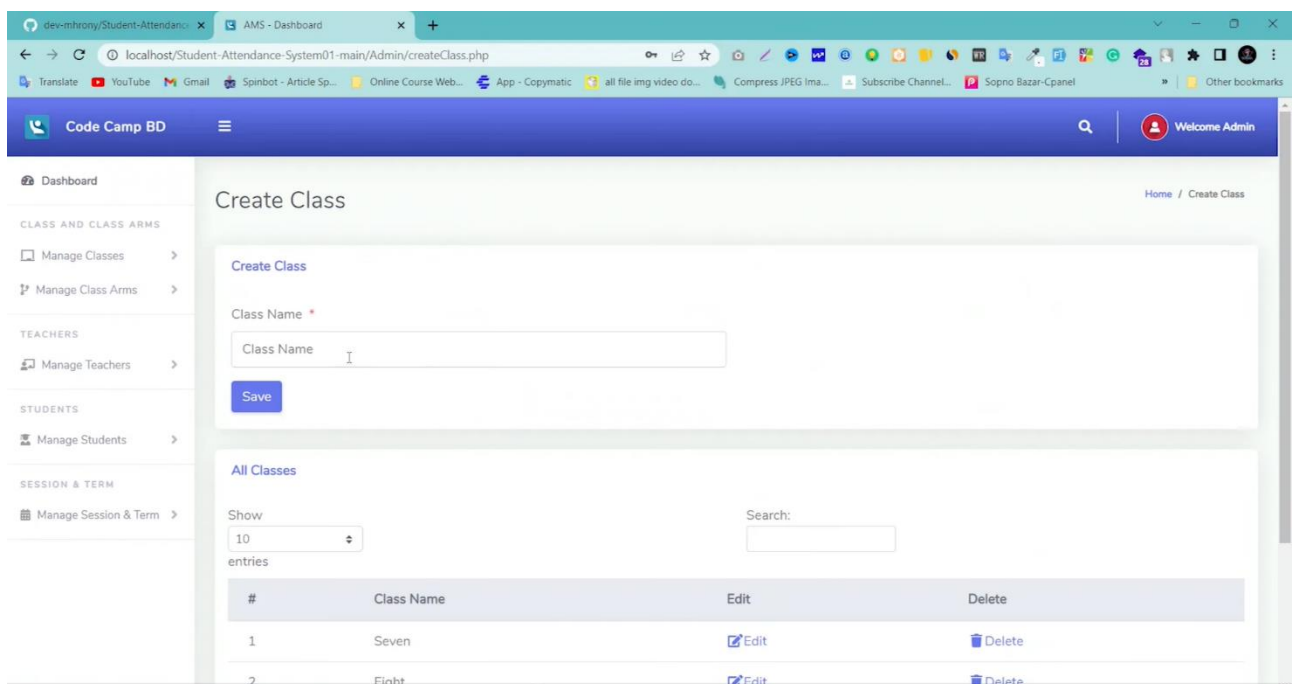
Fig 12 Create Class
