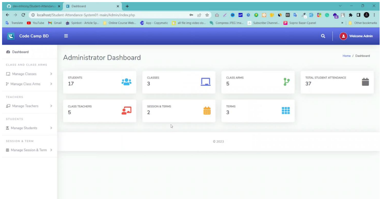
Fig 13 Dashboard
