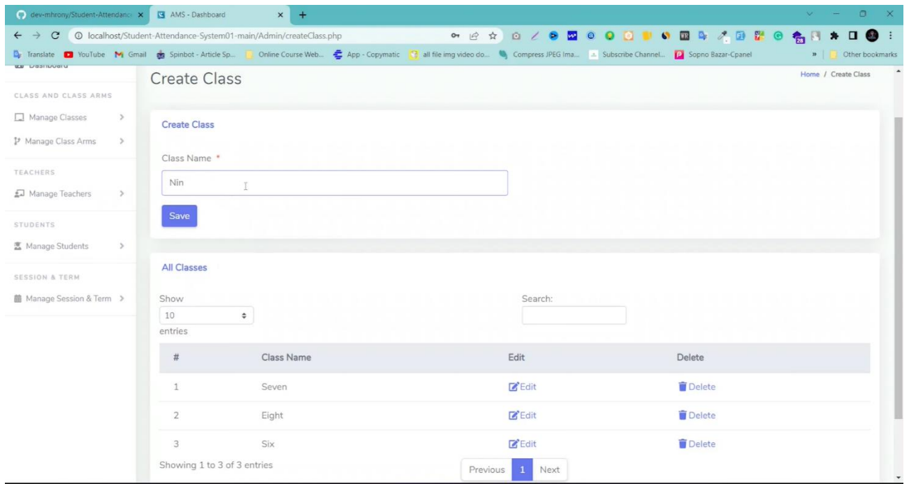
Fig 19 Create Class
