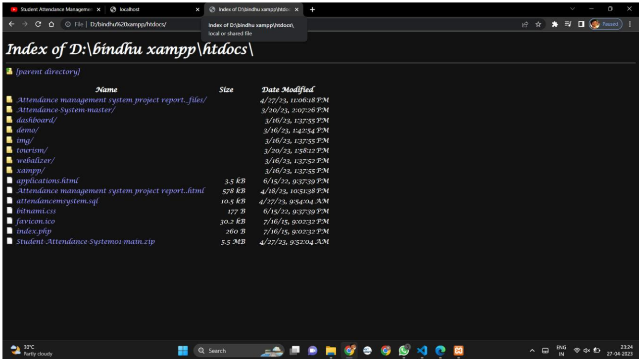
Fig 8 Index Page(1)
