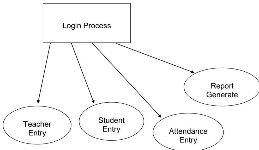
Fig 6 Login Process
