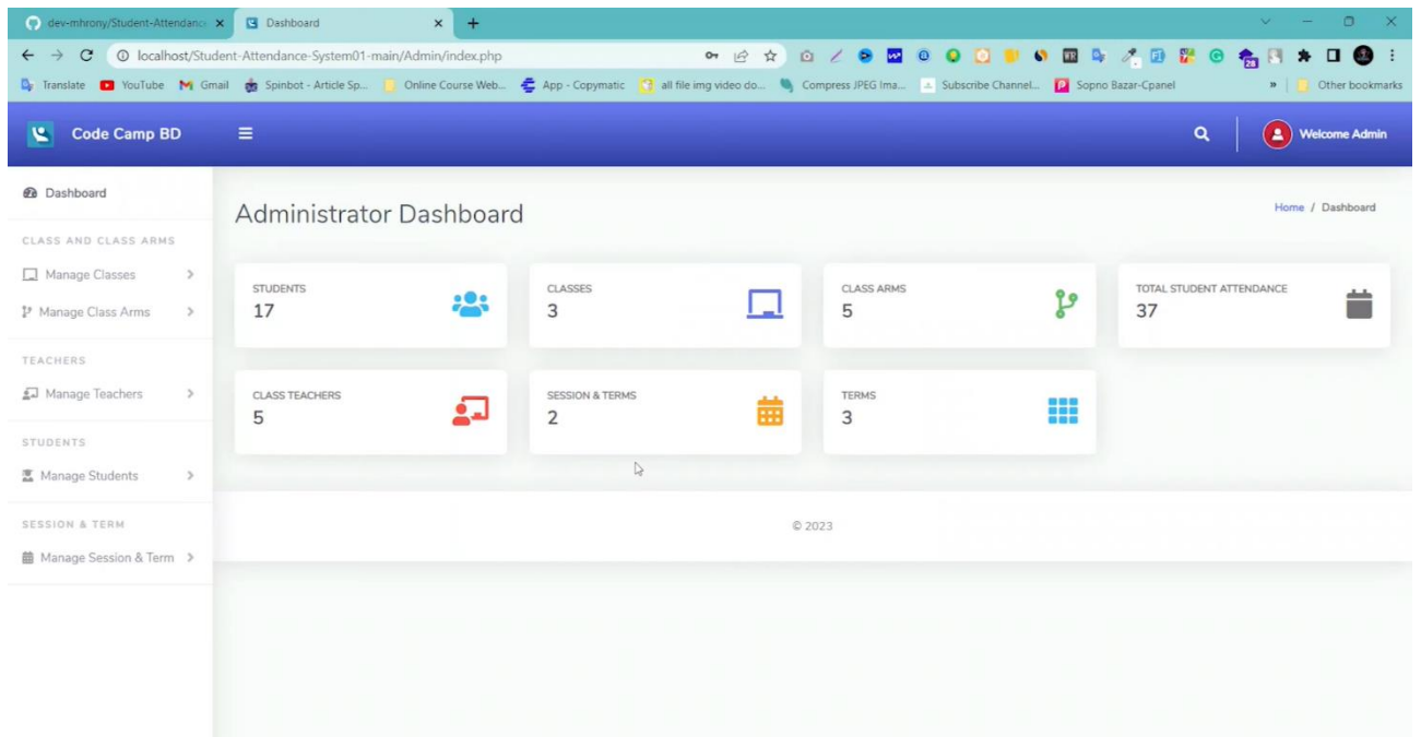
Fig 11 Admin Page
