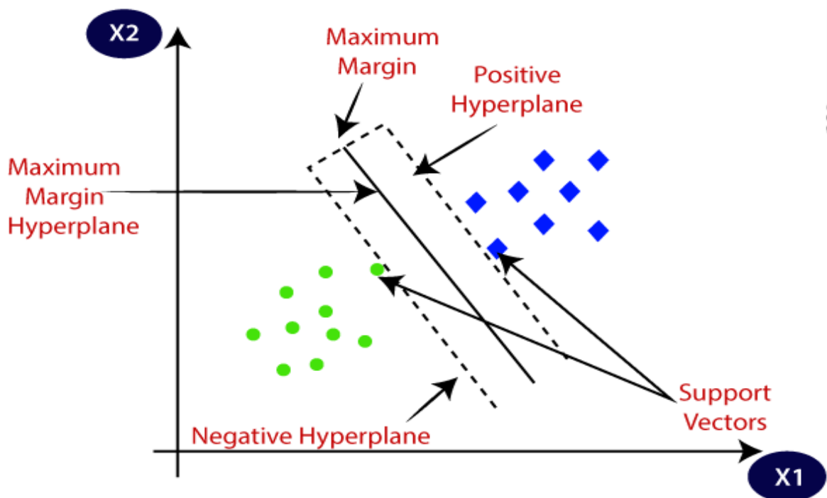
Fig 5.1. Support Vector Machine
