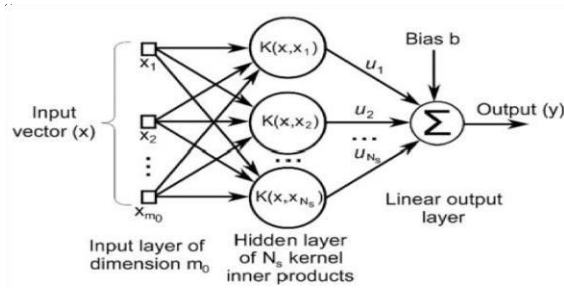
Figure 4: SVM Architecture
