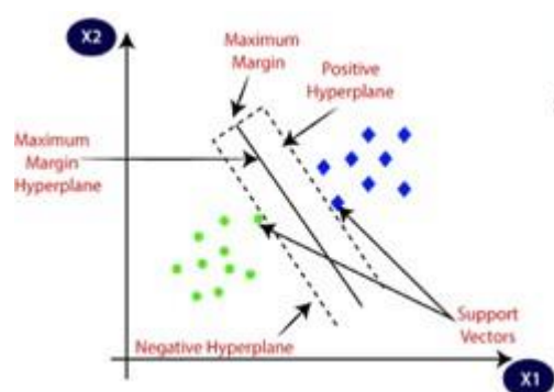
Figure 3: SVM Classification
