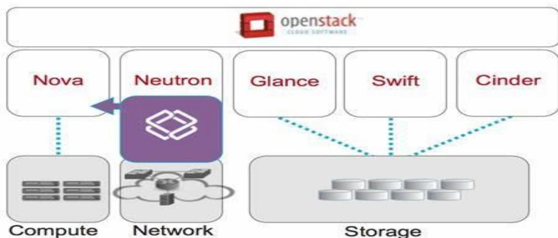
Fig 3.8 OpenStack
