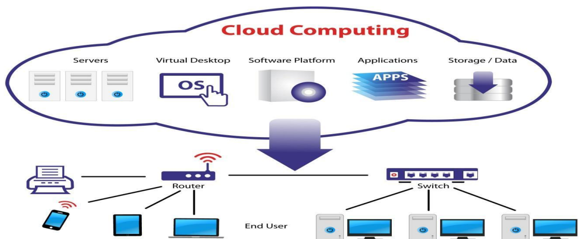
Fig 2.1 Cloud Computing
