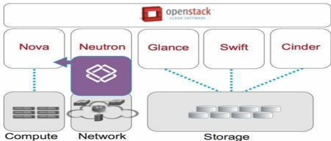
Fig 3.4 OpenStack
