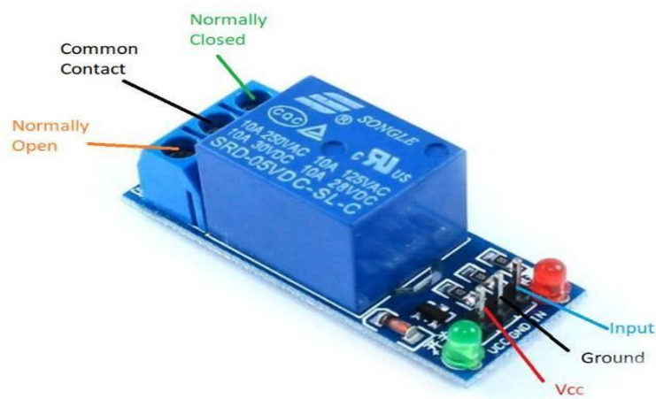
Fig 4.9: Single Channel Relay
