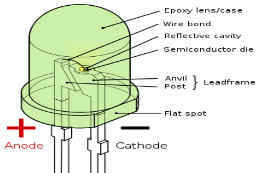
Fig 4.3: Parts of a LED
