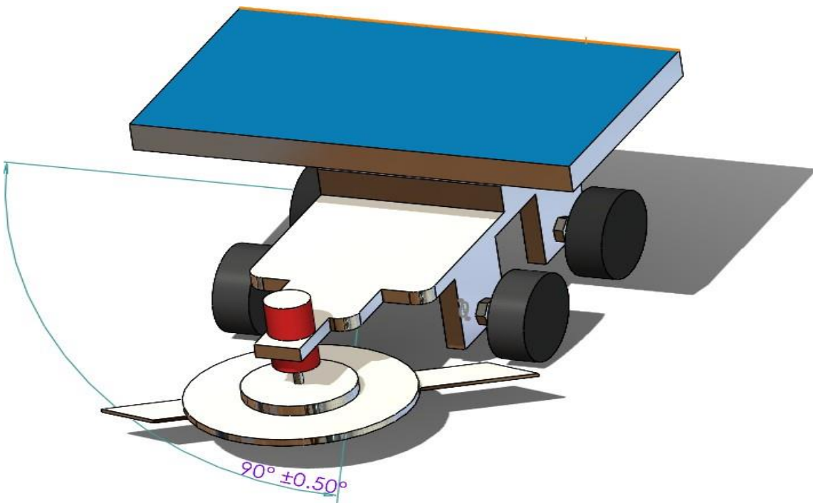
Fig 3.5: overall View
