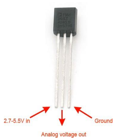
Fig 4.6: Temperature Sensor (LM 35)
