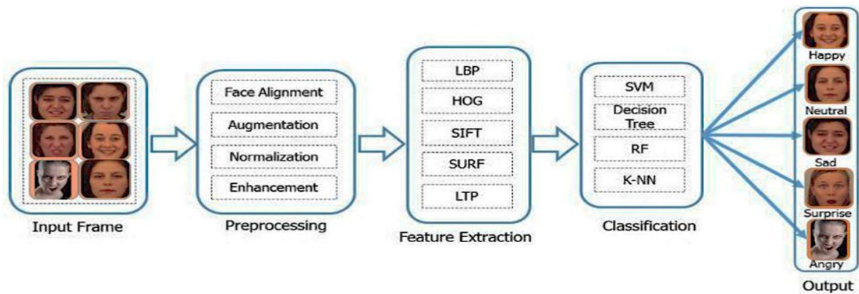
Fig 4.1 Facial Feature Extraction
