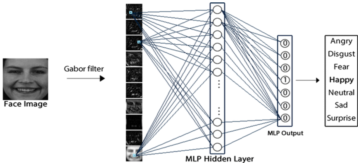
Fig 4.3 MLP classifier classifying emotions
