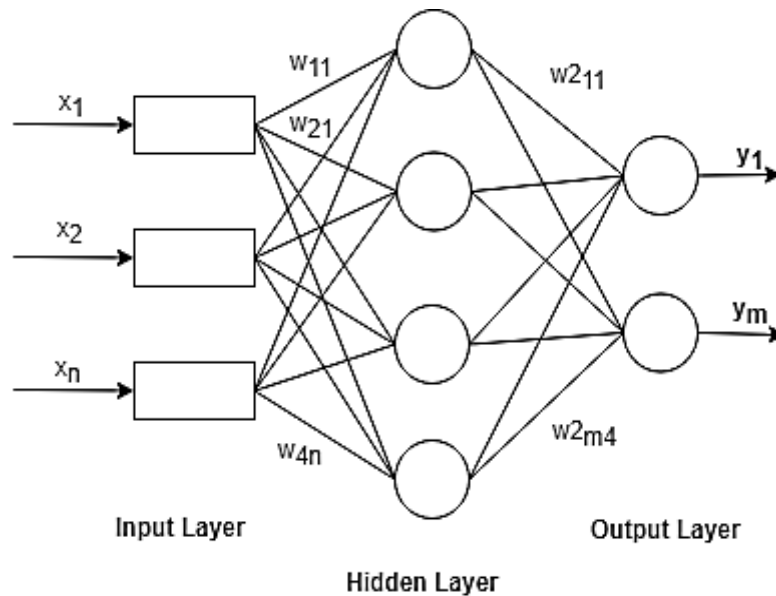
Fig 4.2 MLP hyperparameters
