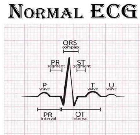
FIG 1.2: ECG WAVEFORM
