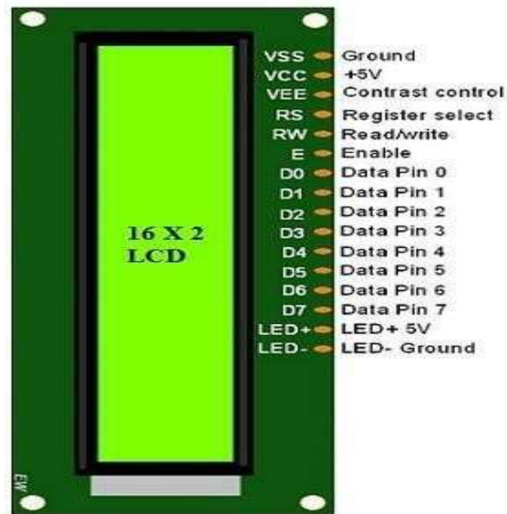
Fig:4.7: 16x2 lcd display pin diagram
