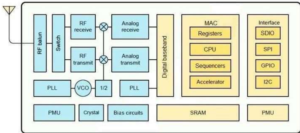
FIG 4.12: BLOCK DIAGRAM OF ESP8266
