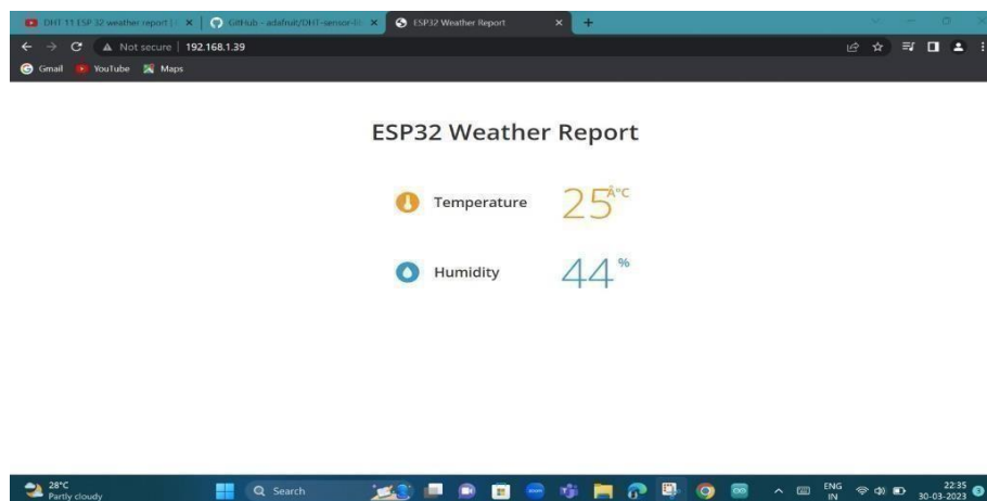
FIGURE 4.4 : OUTPUT CALCULATING PATIENT ROOM TEMPERATURE AND HUMIDITY
