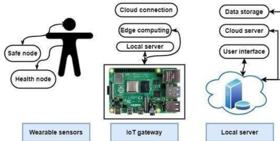
FIGURE 1.4 : Healthcare-monitoring system using wearable sensor
