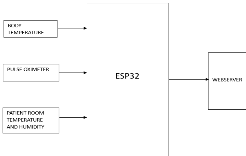
FIGURE 3.1 : BLOCK DIAGRAM OF PROPOSED MONITORING SYSTEM
