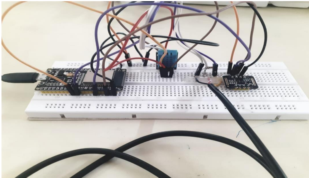
FIGURE 4.5 : HARDWARE CONNECTION OF HEALTH MONITORING SYSTEM
