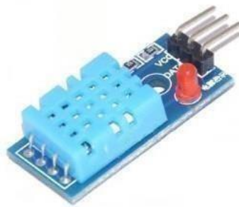
FIGURE 3.5 : TEMPERATURE AND HUMIDITY SENSOR (DHT11)
