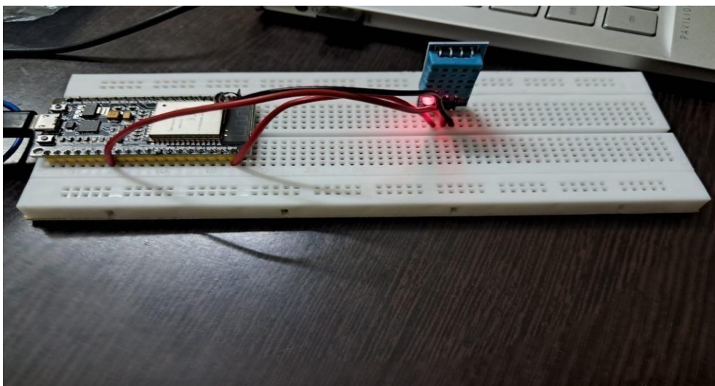
FIGURE 4.3 : TESTING DHT11 SENSOR FOR ROOM TEMPERATURE AND HUMIDITY
